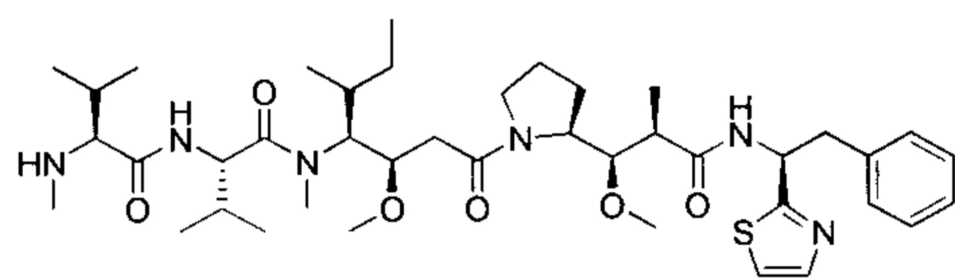
Monomethyl Dolastatin 10 (MMAD)
