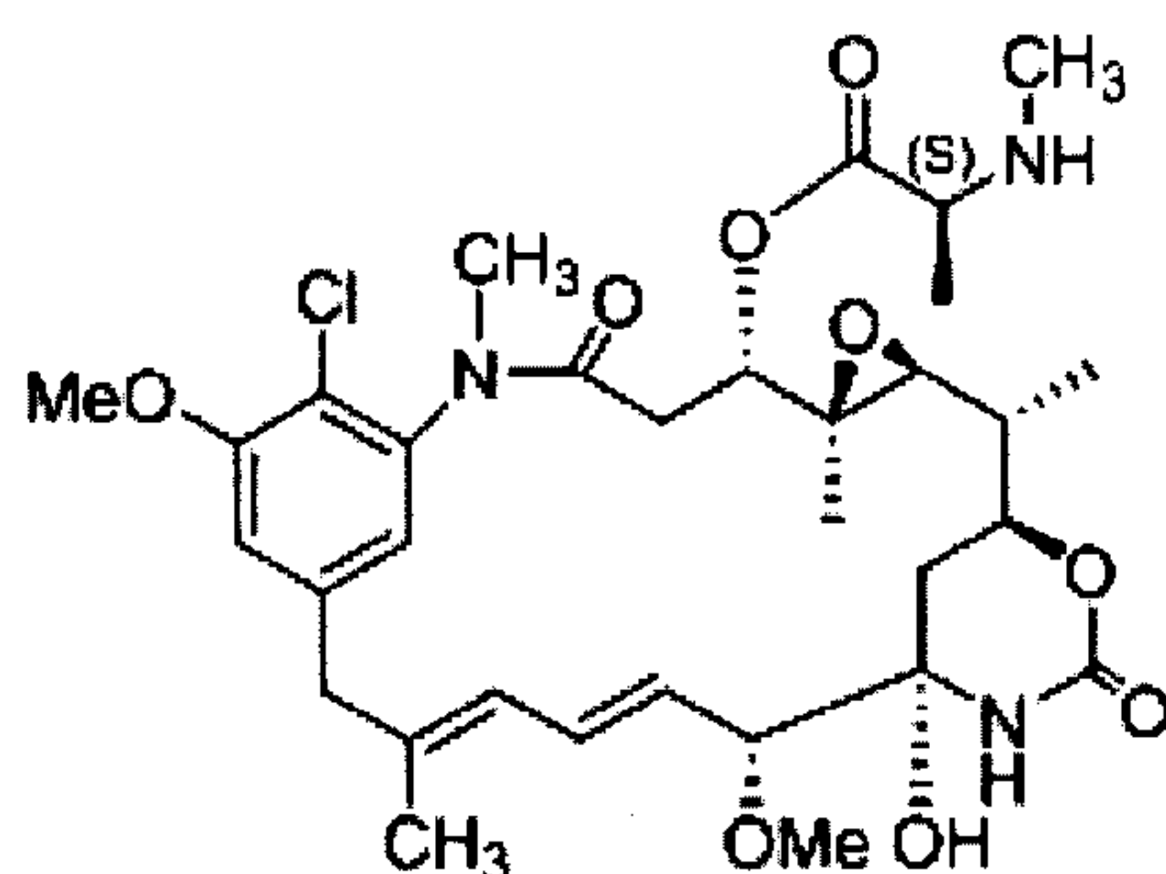
Deacetyl-maytansine
