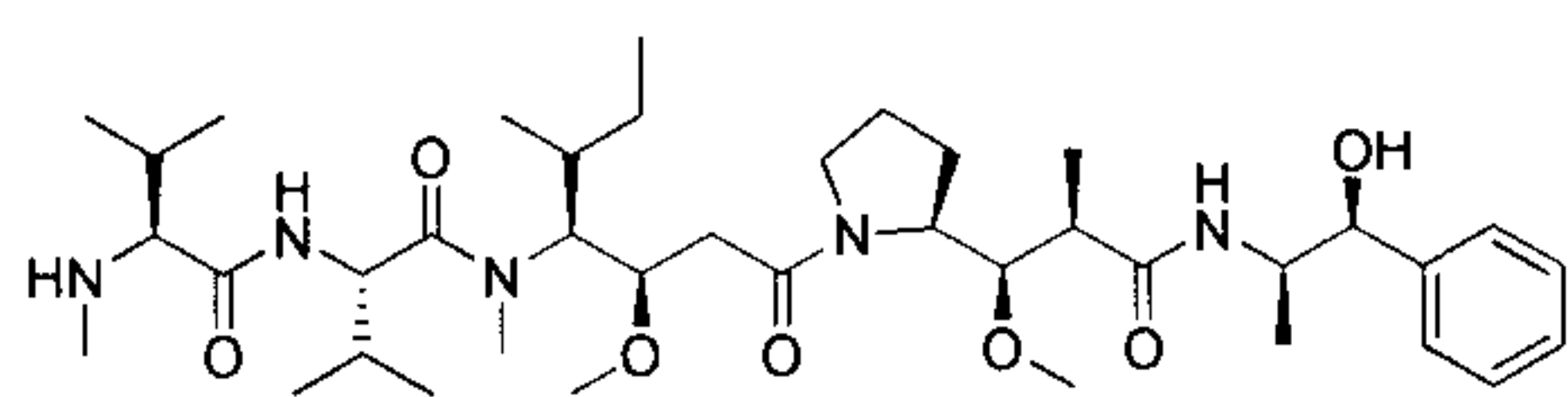
Monomethyl Auristatin E (MMAE)
