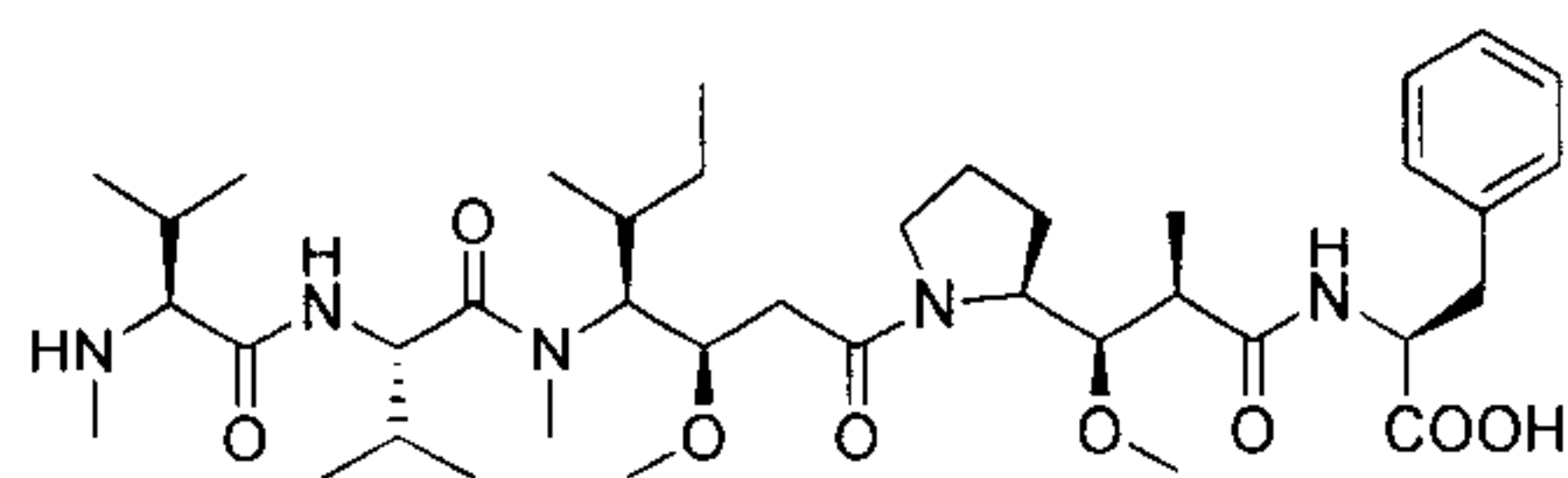
Monomethyl Auristatin F (MMAF)
