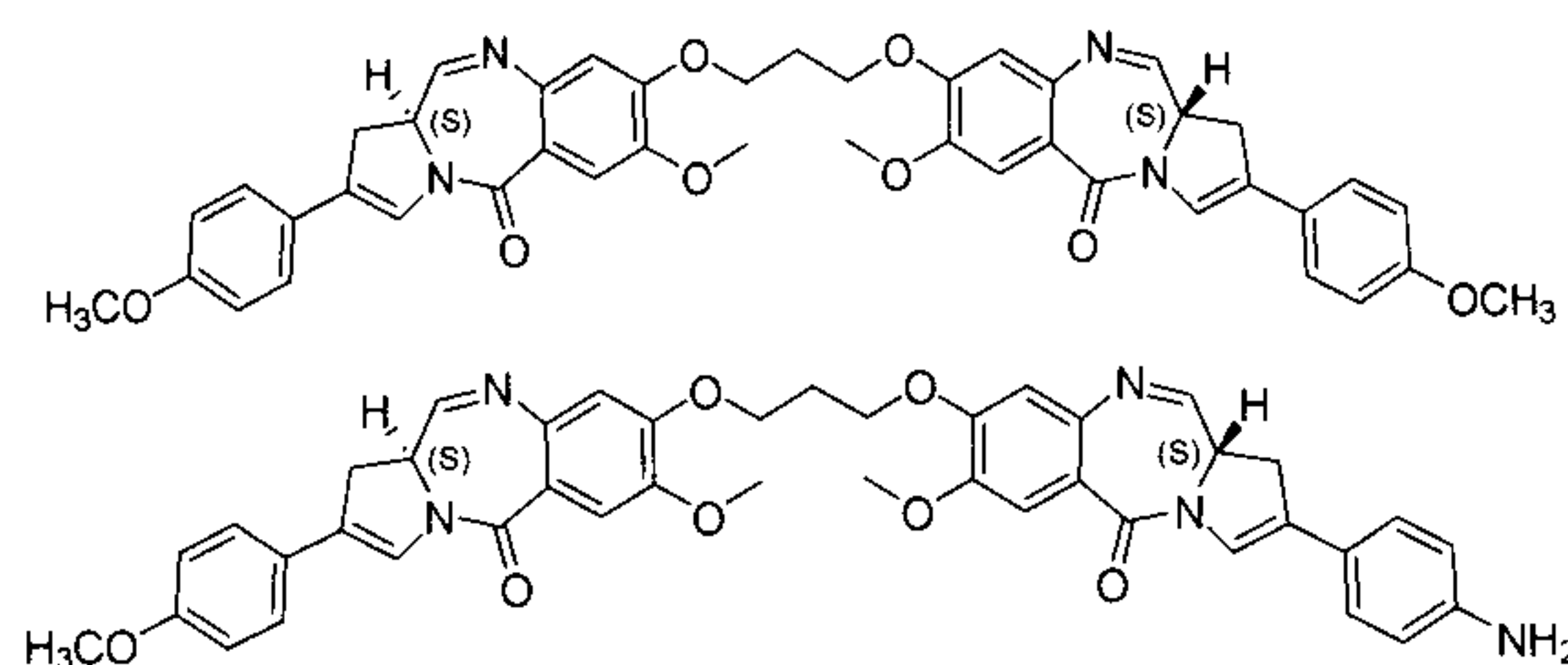
PBD dimers
