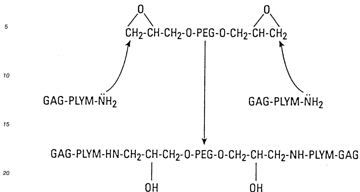
FORMULA 7
