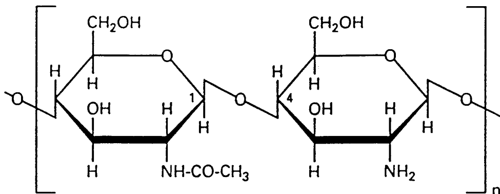
N-Acetylglucosamine
