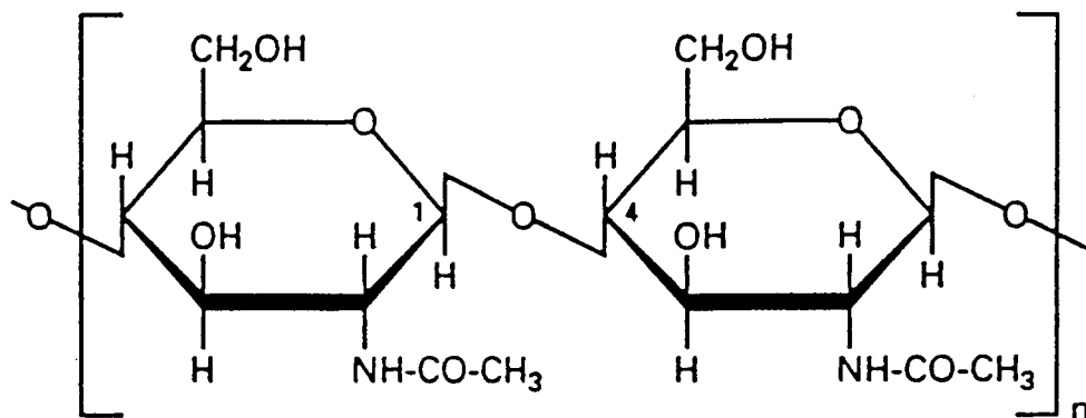
N-Acetylglucosamine
