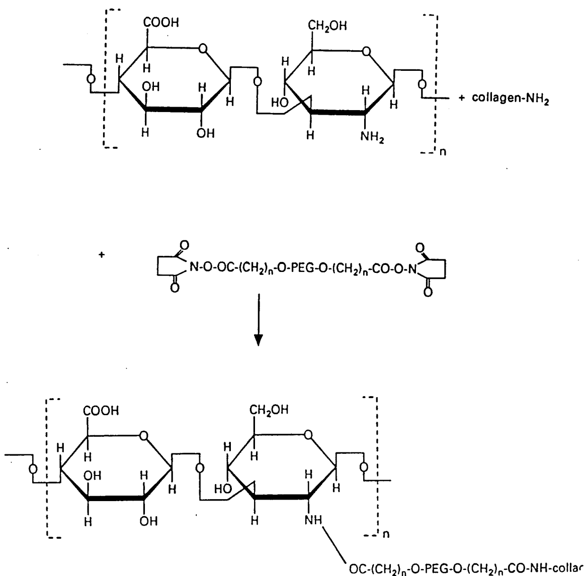
Reaction Scheme 6
