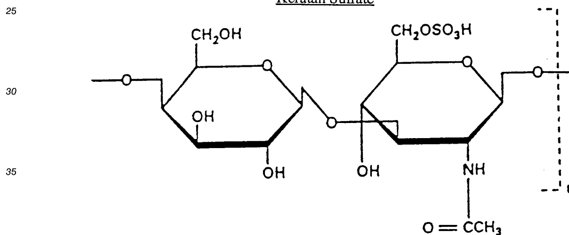
Repeating unit of keratan sulfate
