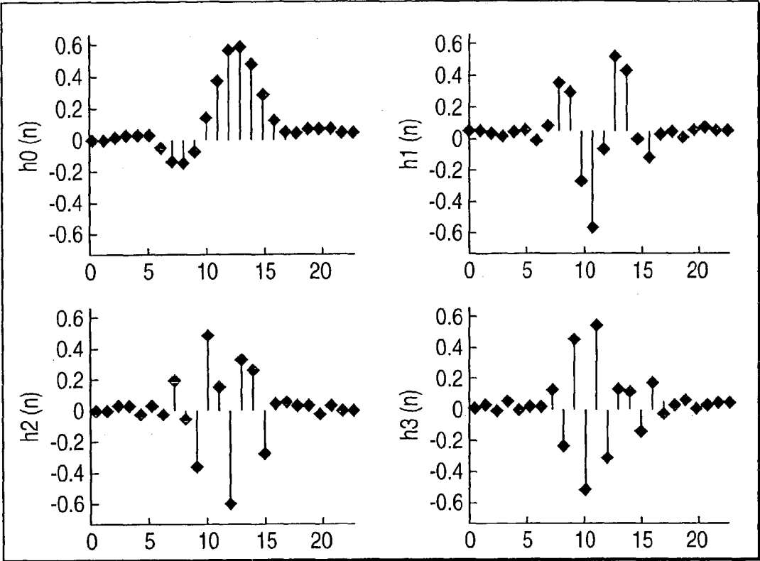
FIG. 11A IMPULSE RESPONSE EXAMPLE OF ELT FILTER BANK (4 DIVISION)
