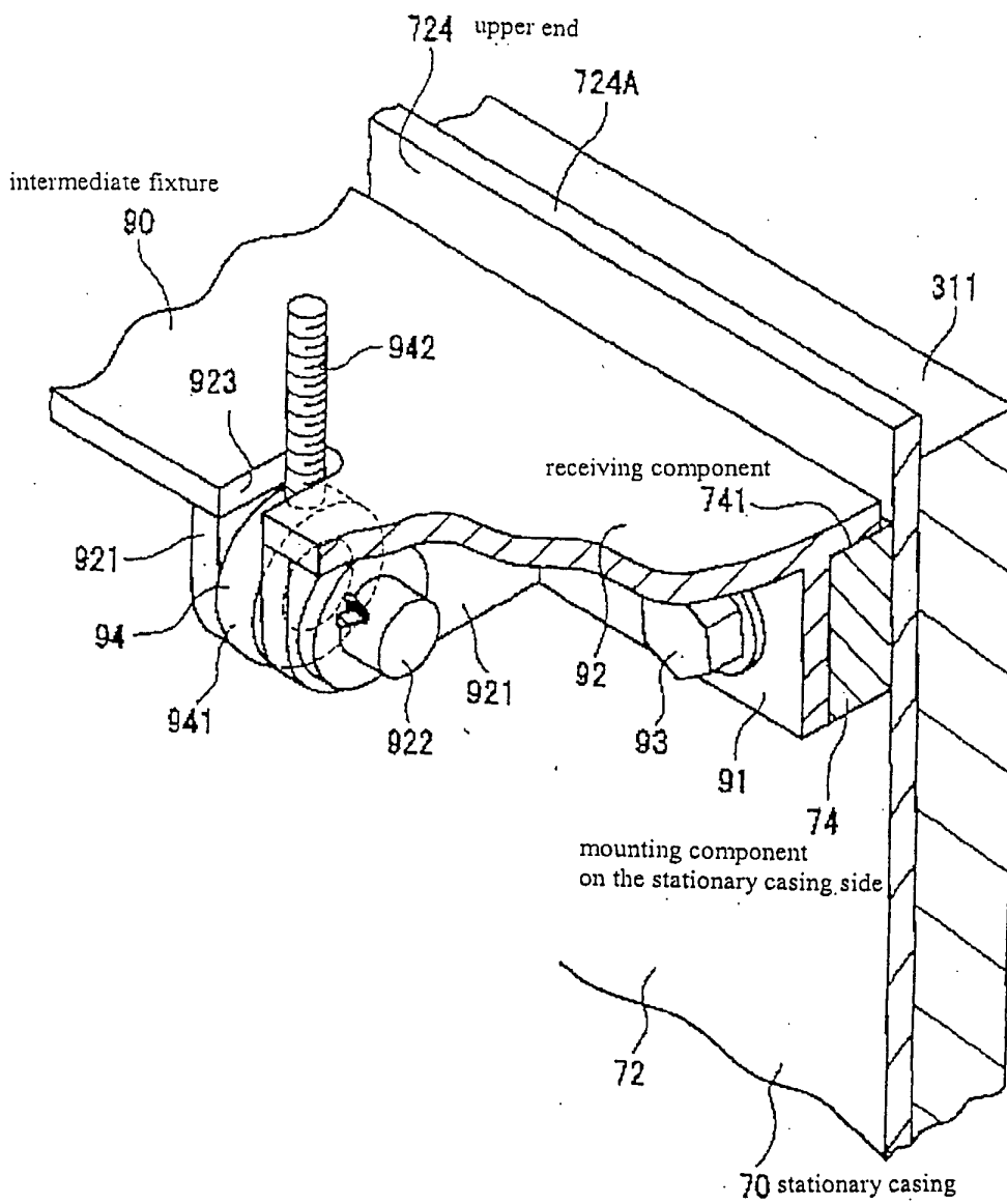
Perspective View Showing the Intermediate Fixture Used for the Casing
