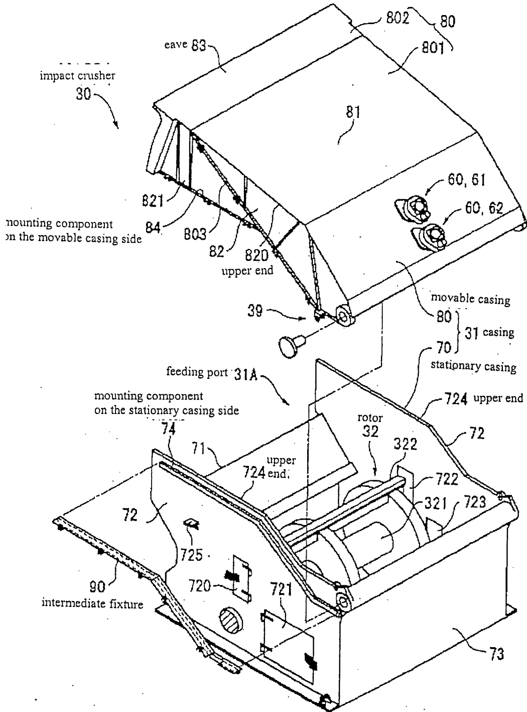
Exploded Perspective View of the Crusher
