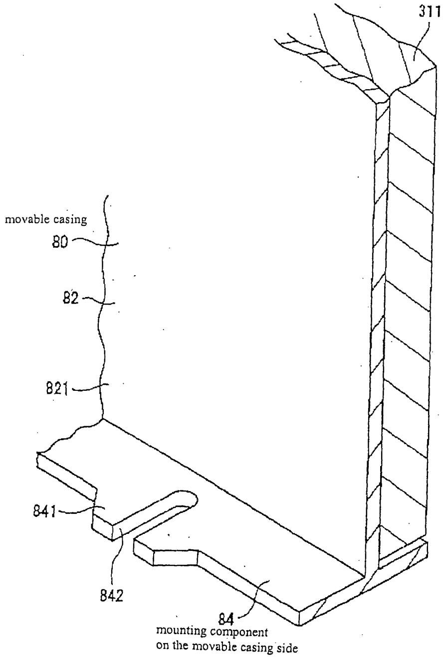
Perspective View Showing a Major Section of the Movable Casing
