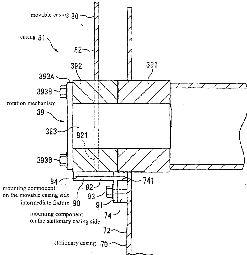
Cross section Showing the Major Section of the Casing of Figure 4
