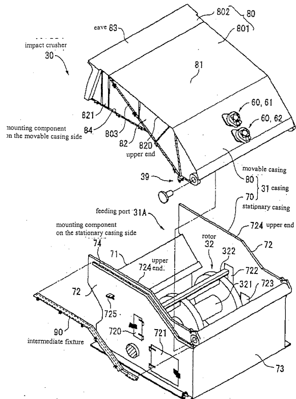
Figure 6 Exploded Perspective View of the Crusher
