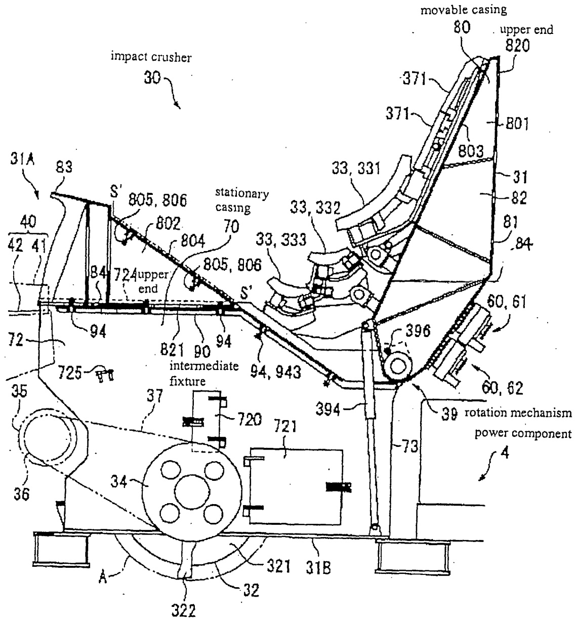
Side View Showing the Movable Casing in the Liner Exchange Position
