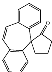
Spiro[cyclopentane-1,5'-[5H]dibenzo[a,d]cyclohepten]-2-one
