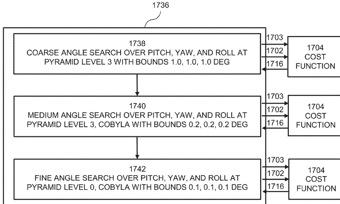
FIG. 17C-2 ANGLE-SEARCH PROCESS 1736
