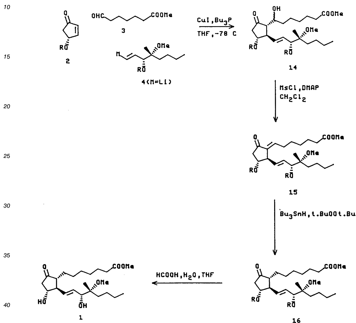
Reaction Scheme C:
