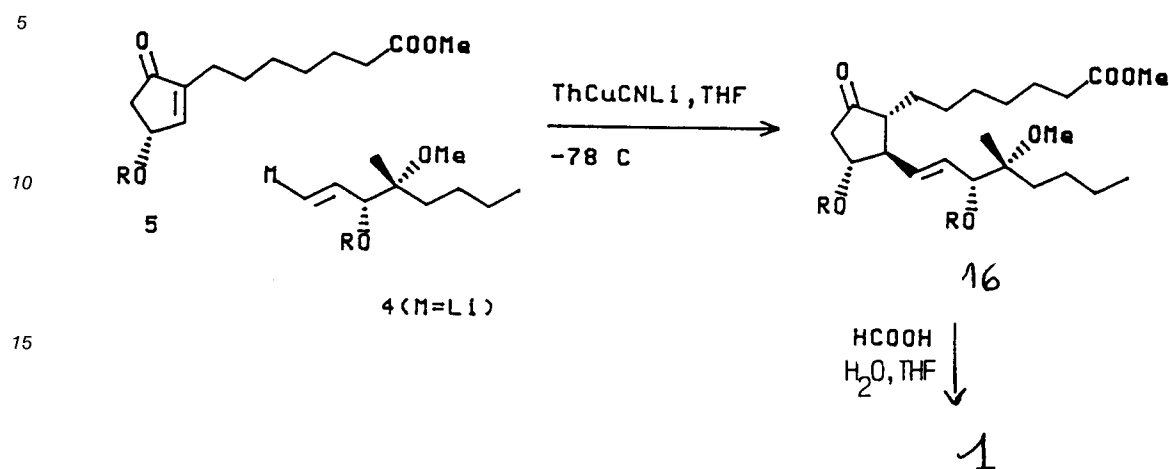
Reaction Scheme D
