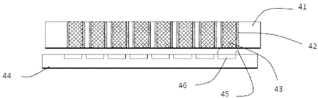
FIG. 4 (PRIOR ART)
