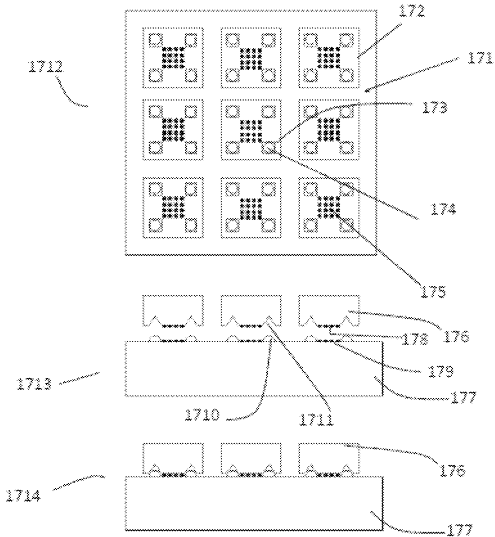
FIG. 17 (PRIOR ART)
