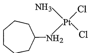
Structural Formula I
