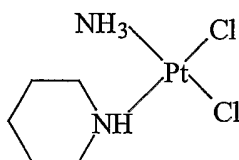
Structural Formula II
