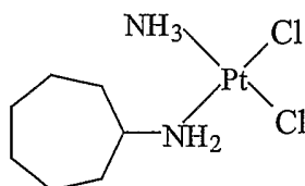
Structural Formula I
