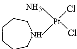
Structural Formula III
