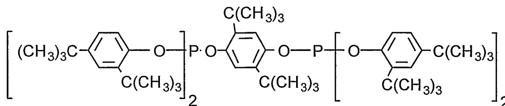
Ligand R
