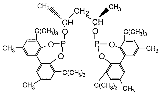
Ligand H
