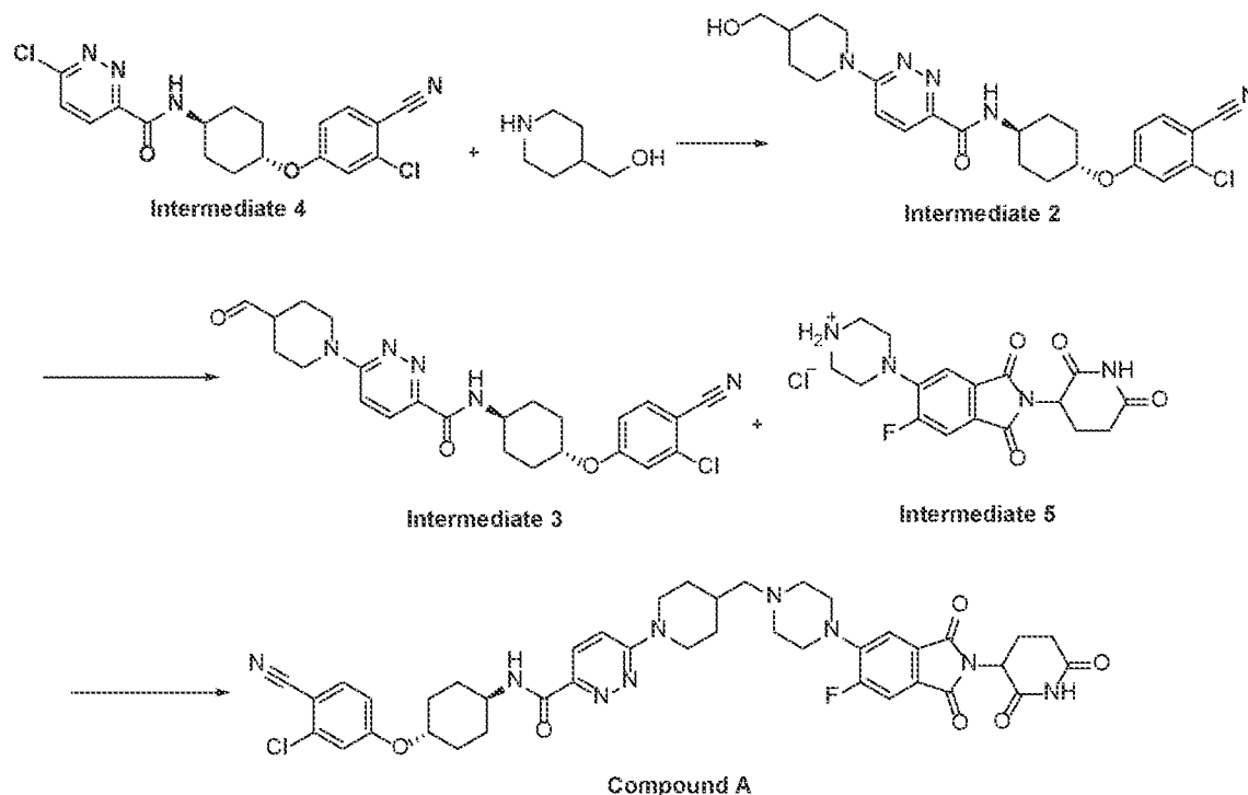
Scheme 4. Second Generation Manufacturing Process of Compound A
