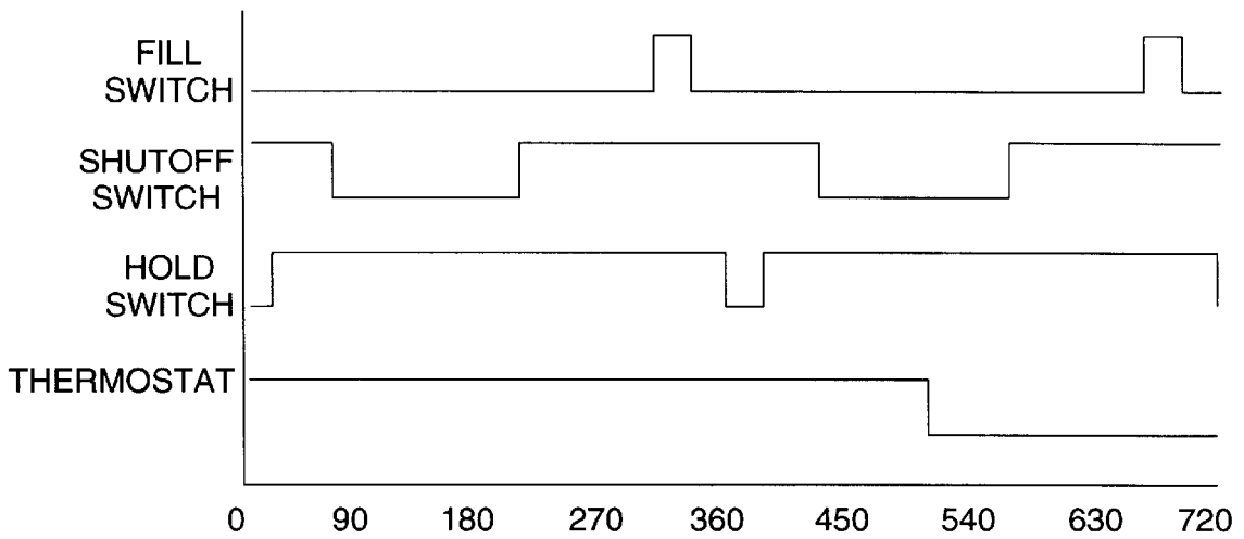
SWITCH STATE DIAGRAM FOR CURRENTLY AVAILABLE ICEMAKERS
