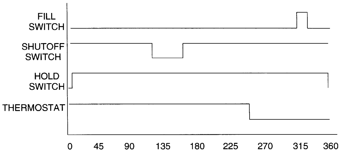
SWITCH STATE DIAGRAM FOR NEW CONTROL CIRCUIT
