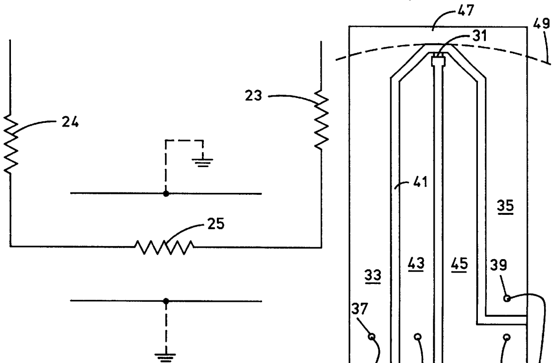
FIG. 4 (Prior Art)
