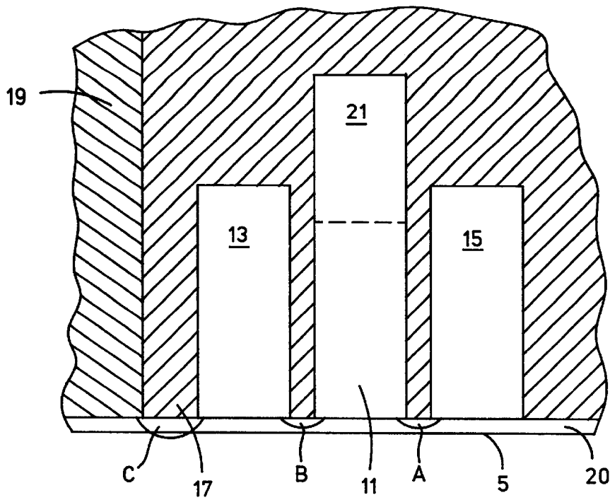
FIG. 3 (Prior Art)
