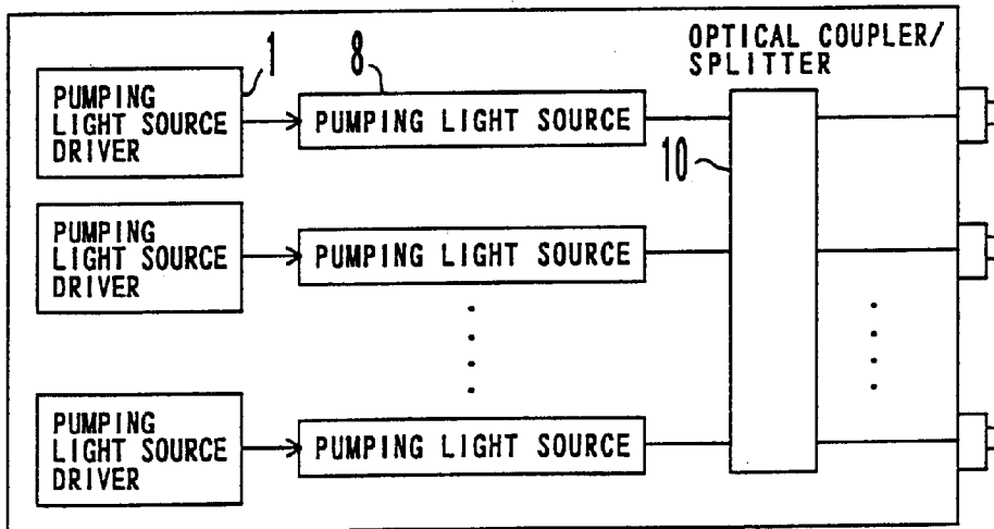
FIG. 1C PRIOR ART
