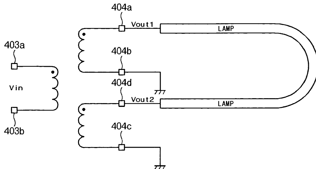
FIG. 4C (PRIOR ART)
