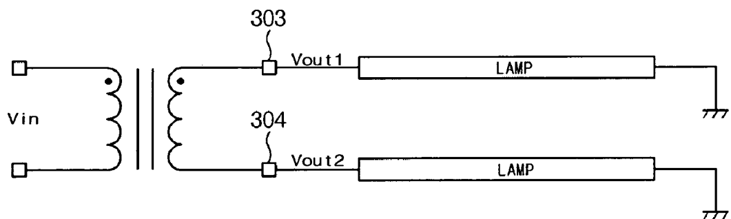
FIG. 3C (PRIOR ART)
