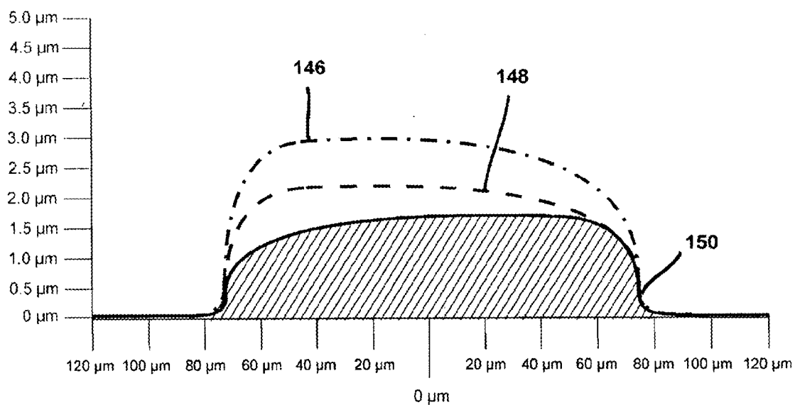
Cross Section Profiles of Bonded / Cured 150 \mu m Wide Lines of Marking Material Compositions Not to Scale
