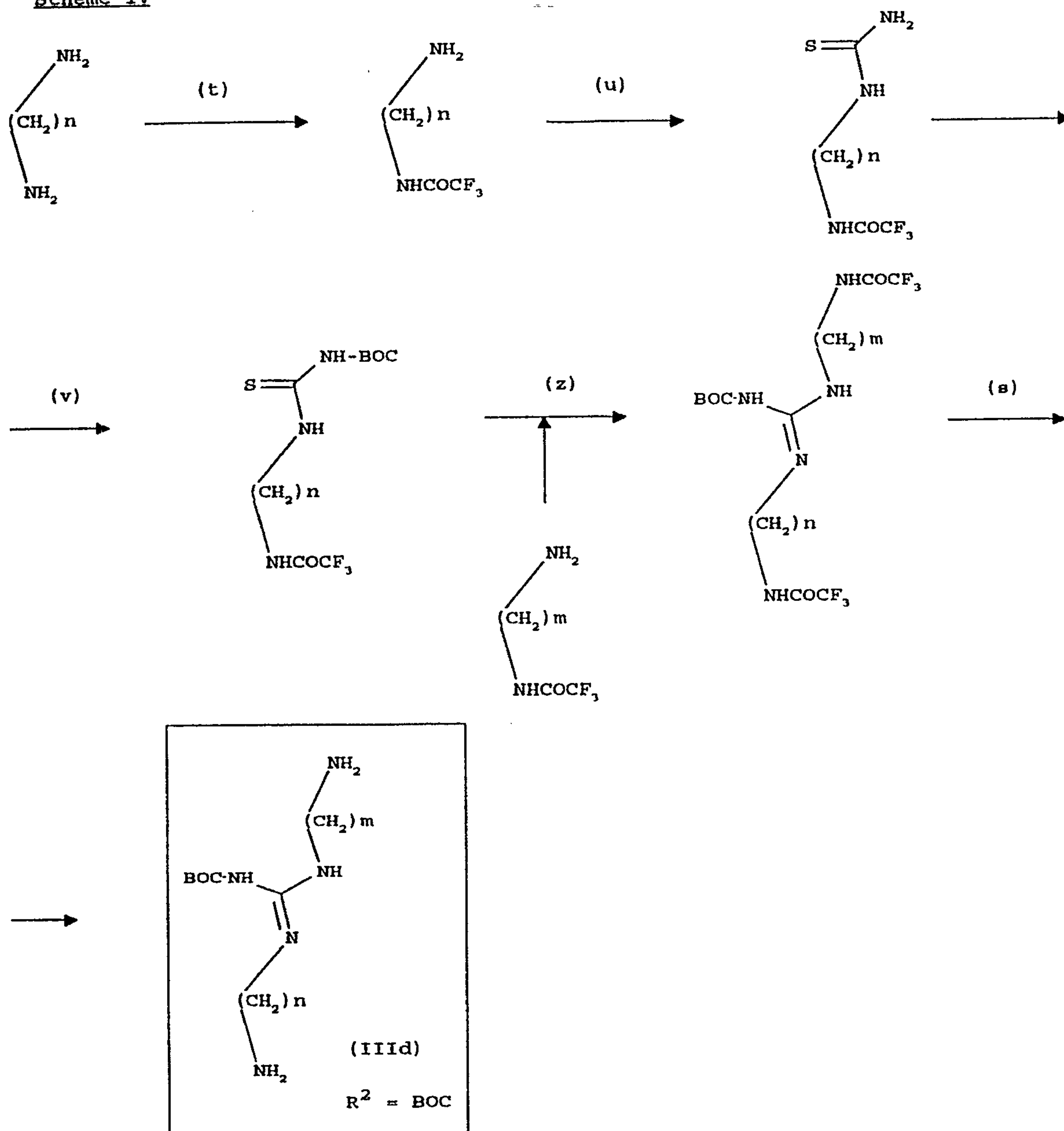
Scheme IV
