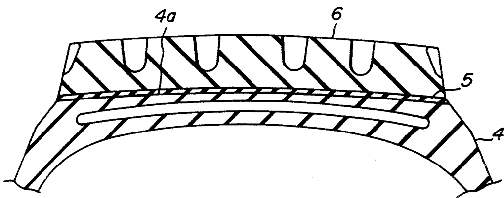
FIG. 20 PRIOR ART
