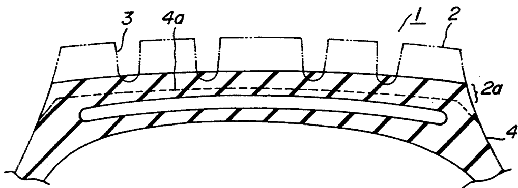
FIG. 19 PRIOR ART
