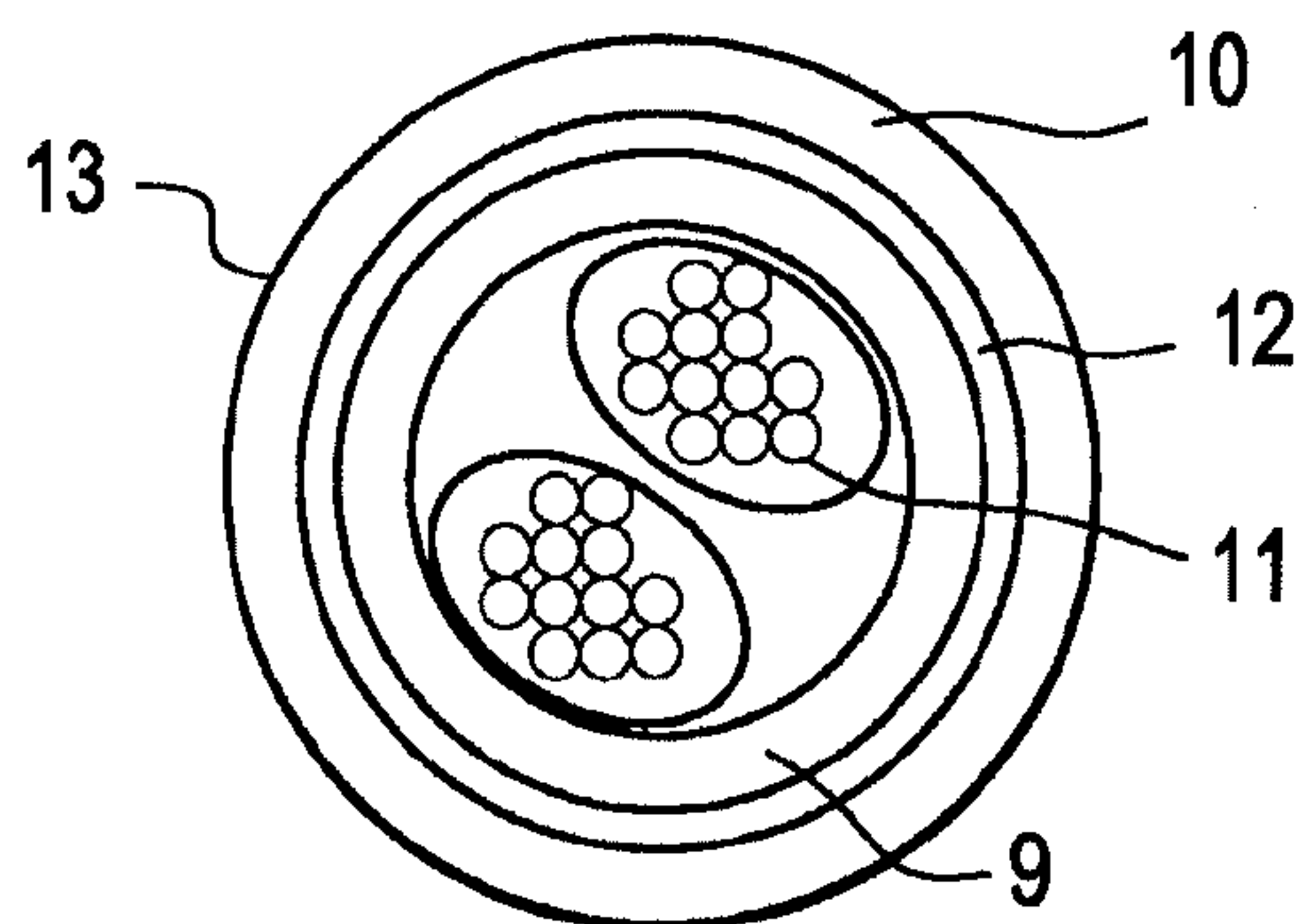
FIG. 3 RELATED ART
