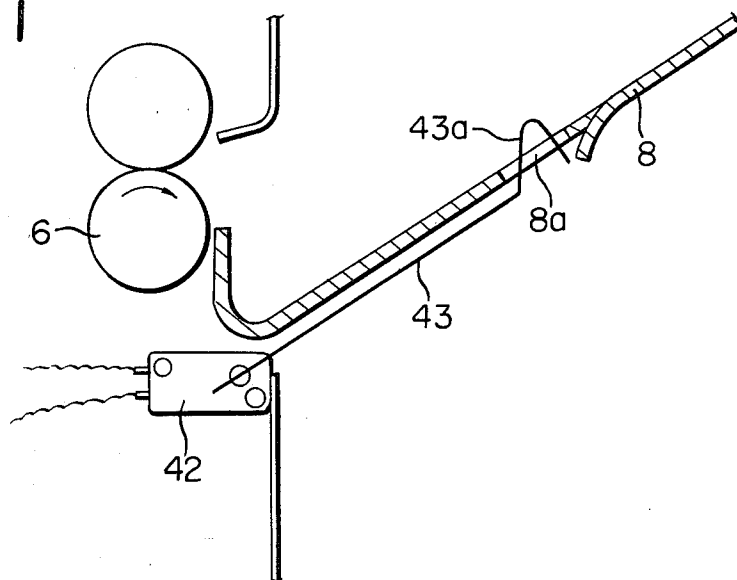
FIG. 12 PRIOR ART
