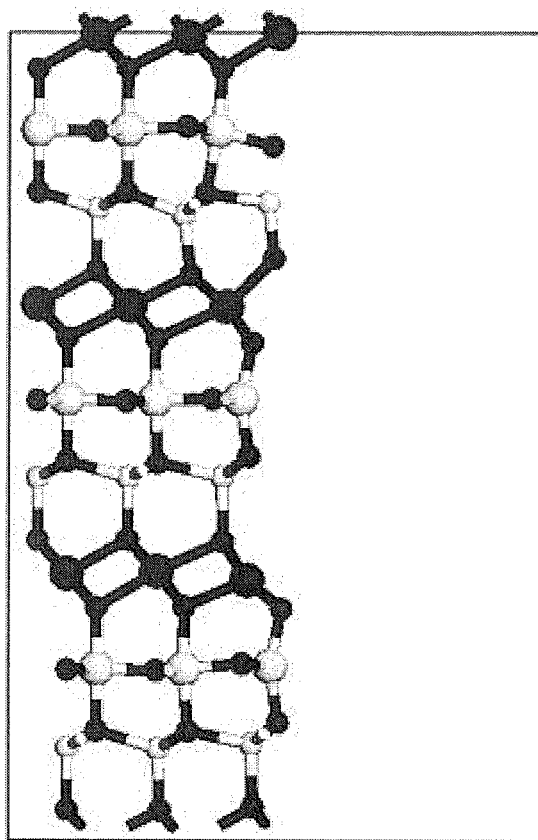
Surface structure (4)
