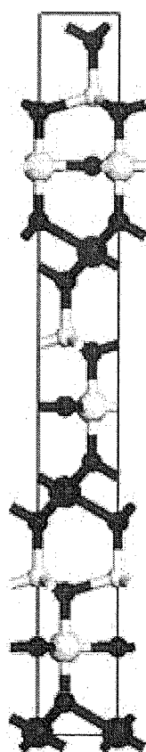
Crystal structure
