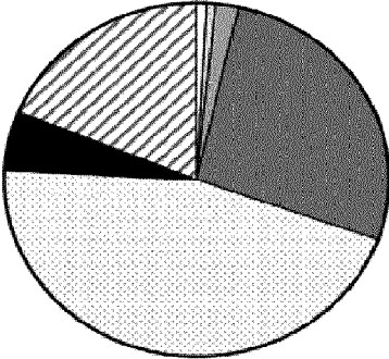
NB B-VLP
