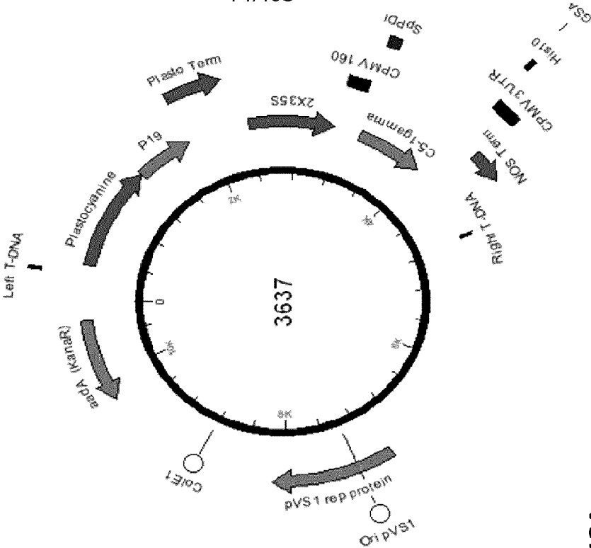
Acceptor construct 3637
