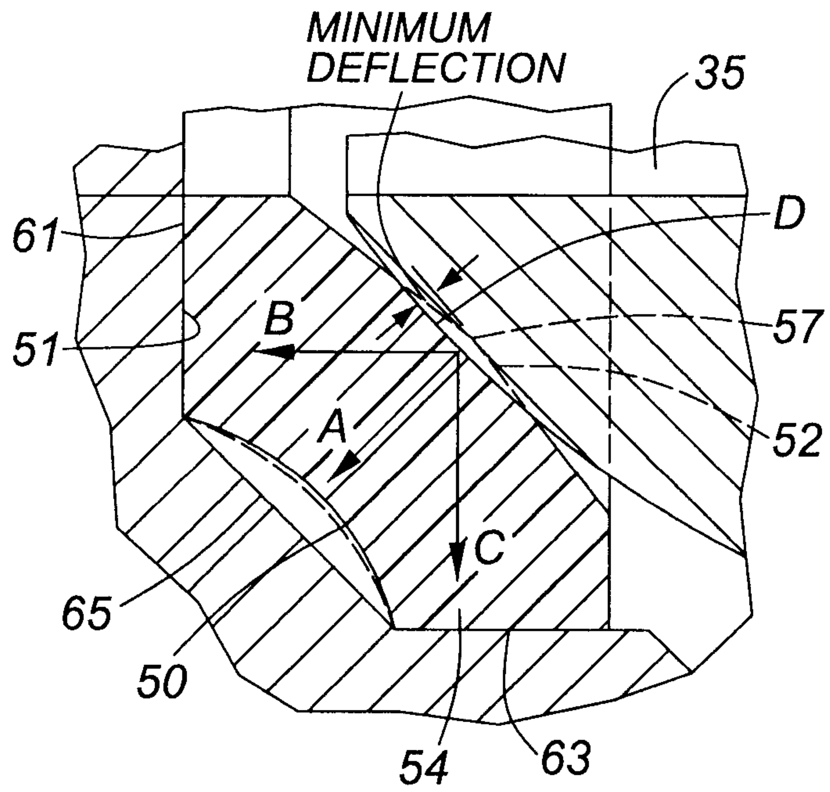
FIG. 3 (PRIOR ART)
