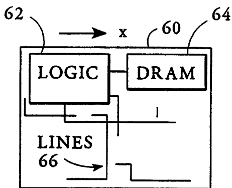
FIG. 5 (Prior Art)
