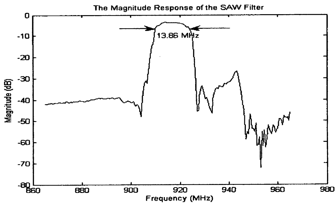
Frequency response of SAW filter
