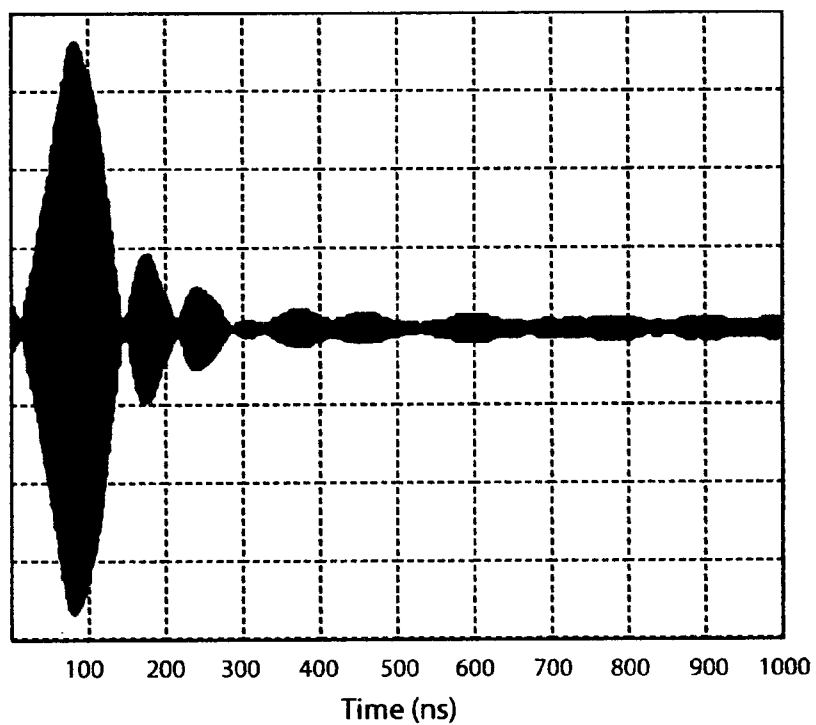
Figure 3 Impulse response of the 14MHz SAW filter
