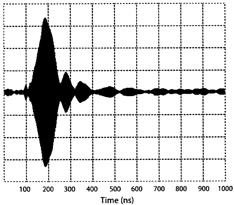
Figure 4 Output response of the 14MHz SAW filter
