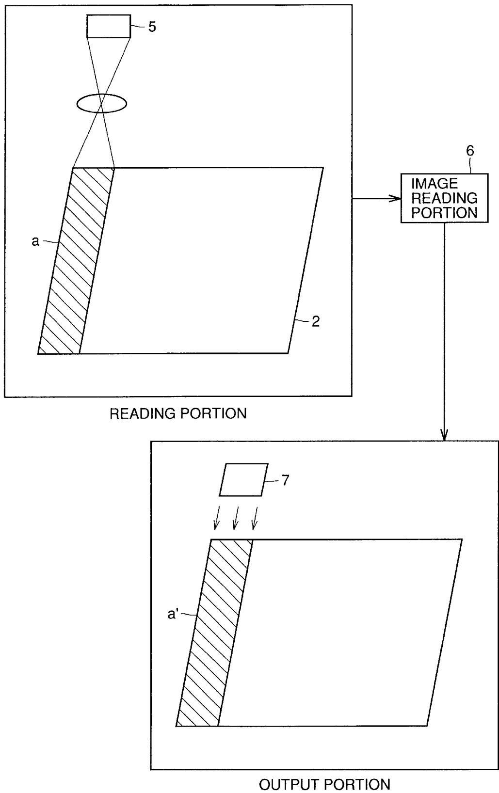
FIG.5 PRIOR ART
