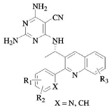
Formula (A)
