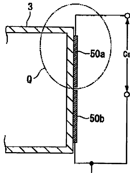
FIG.7B PRIOR ART
