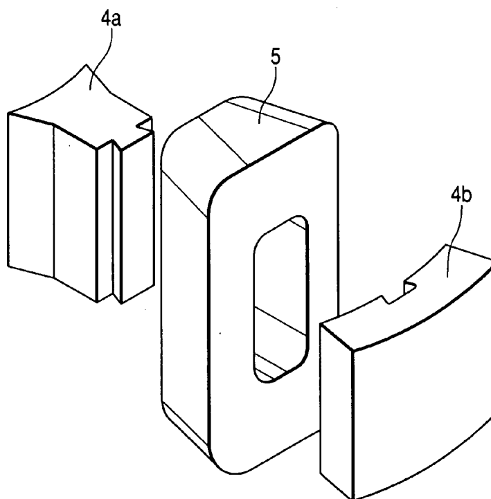
FIG. 19 (PRIOR ART)
