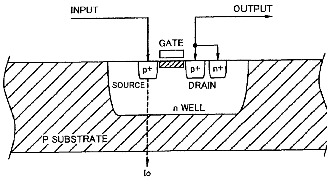
FIG.6 (PRIOR ART)
