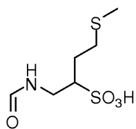
(I-F): 1-formamido-4-(methylthio)butane-2-sulfonic acid;
