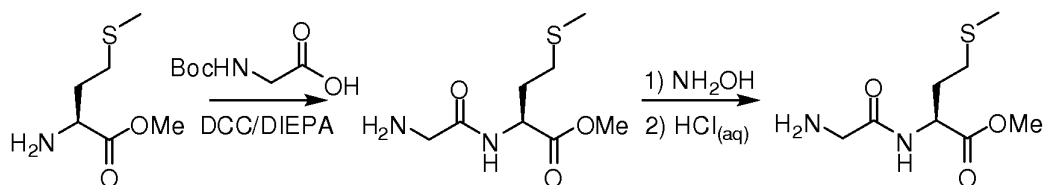
Scheme V
