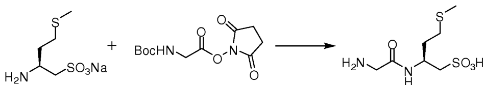
Scheme II
