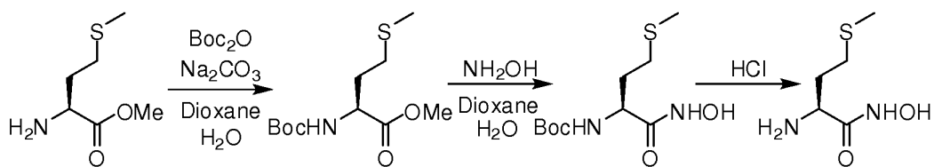
Scheme IV
