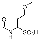
(I-P): 1-formamido-3-methoxypropane-1-sulfonic acid;
