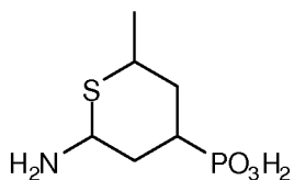
(V-C): 2-amino-6-methyltetrahydro-2H-thiopyran-4-ylphosphonic acid;
