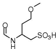
(I-N): 2-formamido-4-methoxybutane-1-sulfonic acid;
