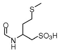
(I-B): 2-formamido-4-(methylthio)butane-1-sulfonic acid;
