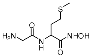
(I-AB): 2-(2-aminoacetamido)-N-hydroxy-4-(methylthio)butanamide;
