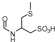
(I-H): 2-formamido-3-(methylthio)propane-1-sulfonic acid;
