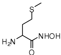
(I-AA): 2-amino-N-hydroxy-4-(methylthio)butanamide;
