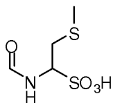
(I-J): 1-formamido-2-(methylthio)ethanesulfonic acid;
