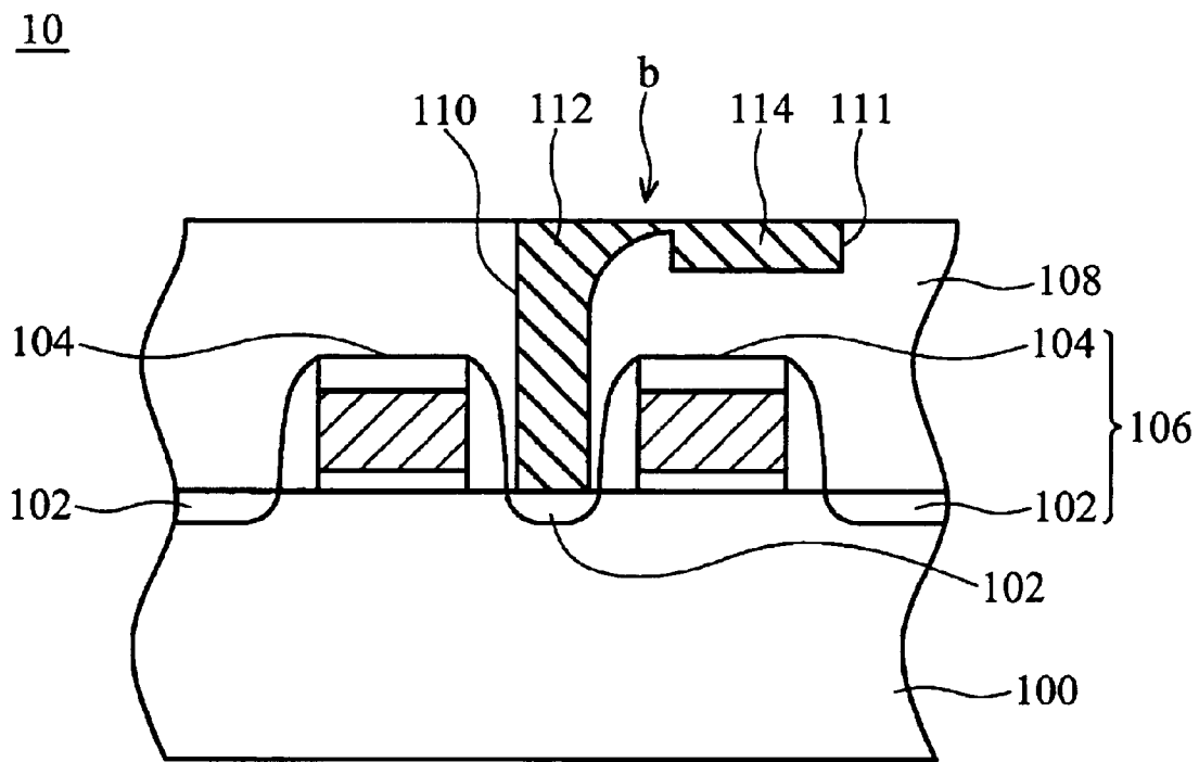
FIG. 1c (RELATED ART)
