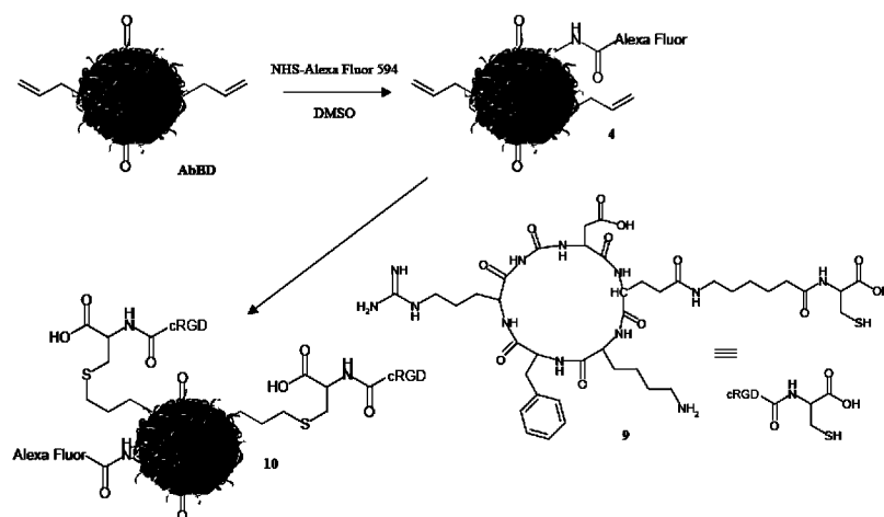
Scheme 23. Attachment of c-RGD
