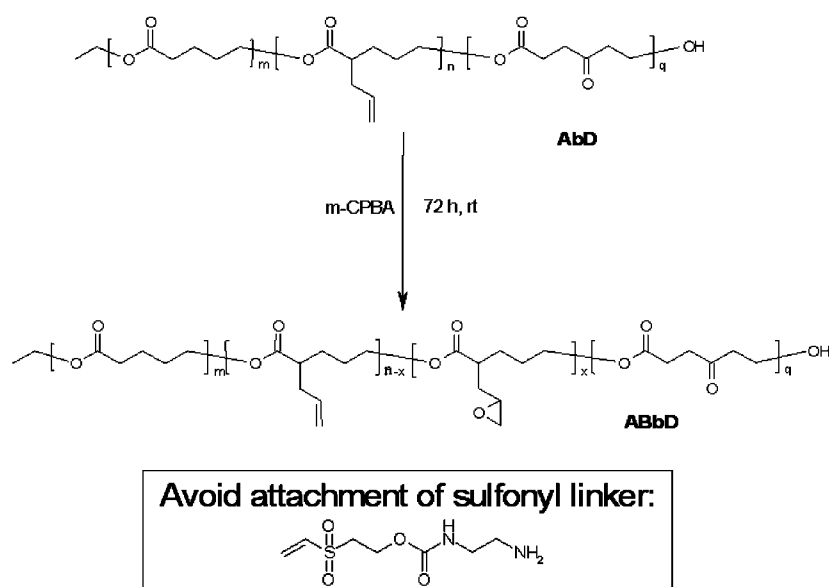
10 Scheme 4. Synthesis of allyl functionalized ABbD linear precursor
