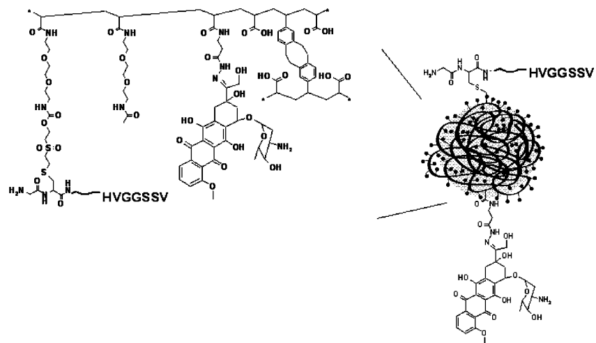
Scheme 15. Attachment of targeting unit; also c-RGD
