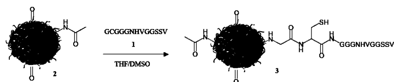
Scheme 9b. Attachment of the targeting peptide to a nanoparticle system.
