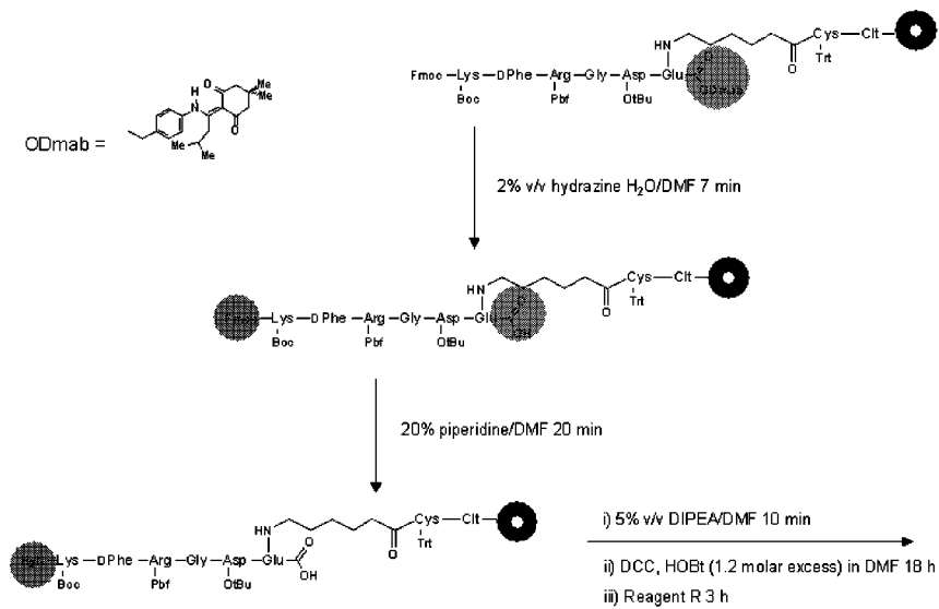
Scheme 17. Synthesis of C-RGD
