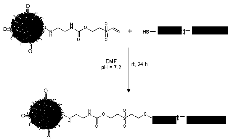
Scheme 2. Attachment of peptide with integrated thiol group from cysteins to linker modified particle
