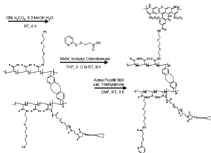
Scheme 20. Further modification of dendrimer functionalized organic quantum dots.
