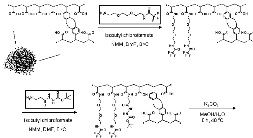
Scheme 12a. DOTA instead of Dye.
