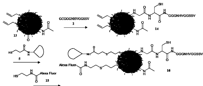
Scheme 26. Synthesis of NP-P-MT-dye conjugate, ABbD-NP-594-MT utilizing reductive amination and thiol-ene chemistry.
