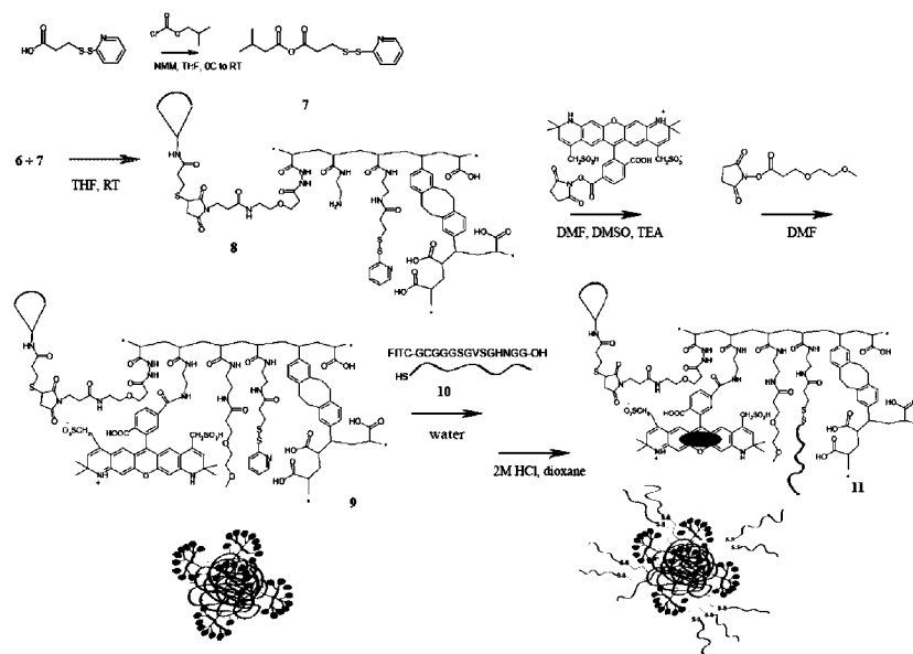
Scheme 8c. Sequential modification of collapsible nanoparticle.
