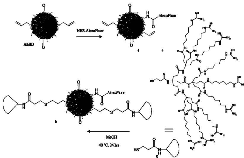
Scheme 12b. Synthesis of delivery of Imaging Reagents to the Eye for Testing.
