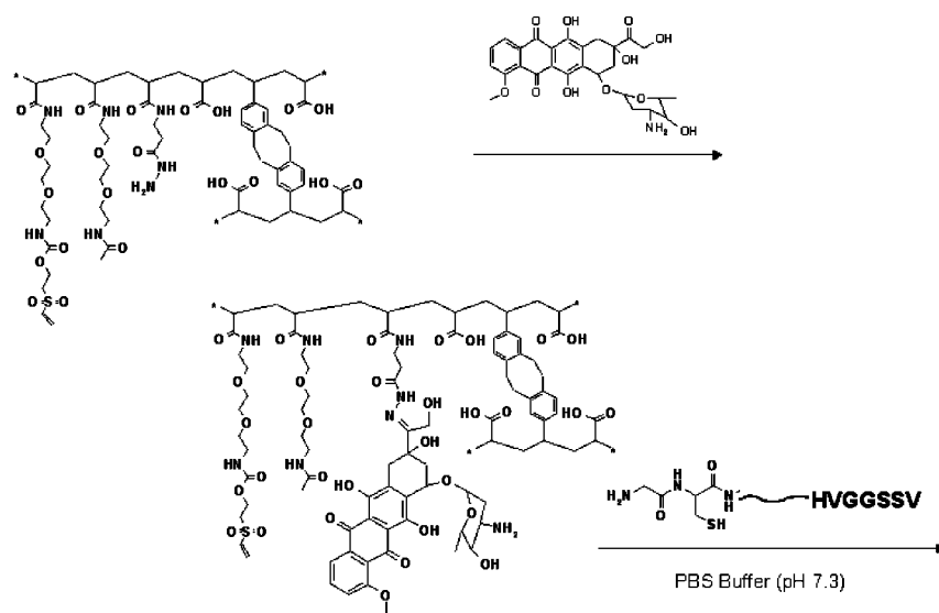
Scheme 14. Hydrazide linker formation of doxorubicine
