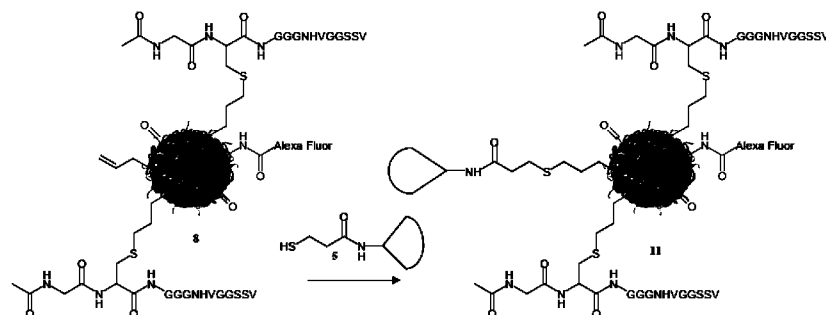
Scheme 24. Combination of dendritic and peptidic scaffold.
