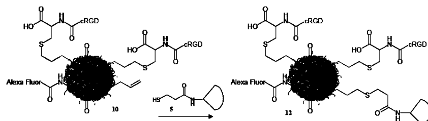
Scheme 25. Synthesis of NP-P-MT-dye, ABbD-NP-594-cRGD-MT (12), utilizing thiol-ene chemistry.
