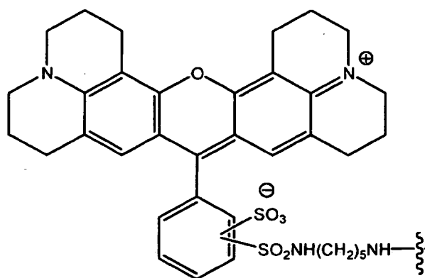
Texas Red-NH-
