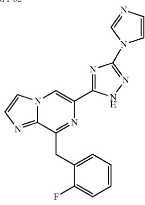
Compound I-63
