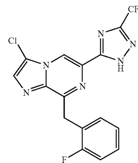
Compound I-67
