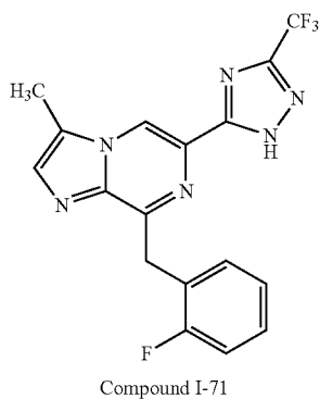
8-(2-Fluorobenzyl)-3-methyl-6-(3-(trifluoromethyl)-1H-1,2,4-triazol-5-yl)imidazo[1,2-a]pyrazine (I-71)
