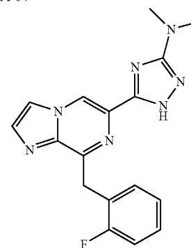
Compound I-65
