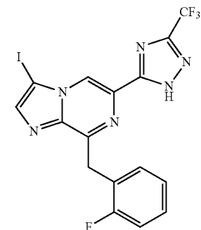
Compound I-66
