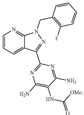
vericiguat (BAY 1021189)
