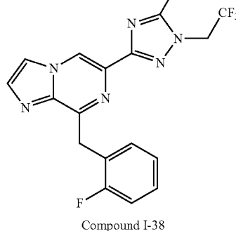
Compound I-38
