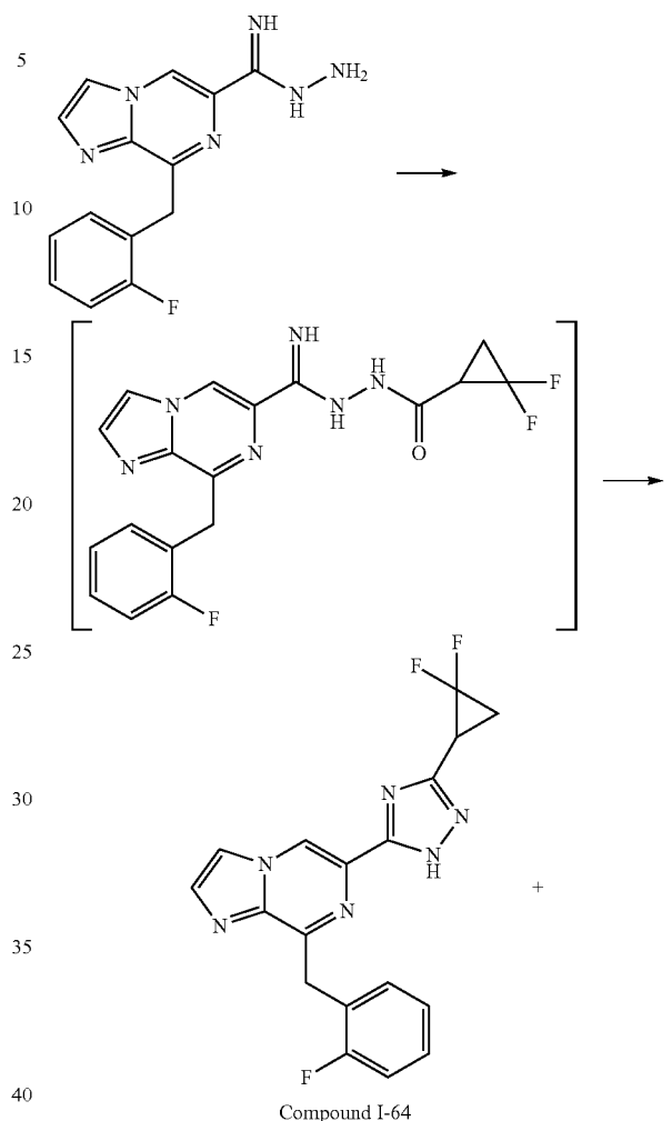
Compound I-64
