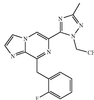
Compound I-39
