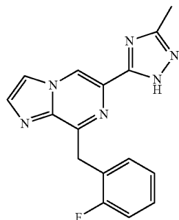
Compound I-4
