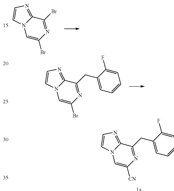
8-(2-Fluorobenzyl)imidazo[1,2-a]pyrazine-6-carbonitrile (1a)
