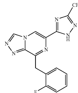
Compound I-72
