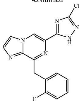
Compound I-62
