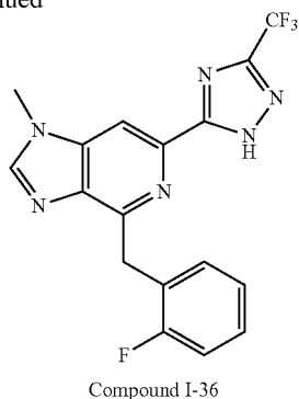
Compound I-36
