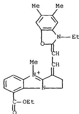
Iodure de 1H-Pyrrolo[1,2-a]benzimidazolium, 8-(ethoxycarbonyl)-3-[(3-ethyl-5,6-dimethyl- 2(3H)-benzoxazolylidene)ethylidene]-2,3- dihydro-4-methyl
