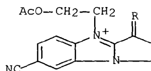
Iodure de 1H-Pyrrolo[1,2-a]benzimidazolium, 8-(ethoxycarbonyl)-3-[(3-ethyl-5,6-dimethyl- 2(3H)-benzoxazolylidene)ethylidene]-2,3- dihydro-4-methyl
