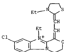
Iodure de 1H-Pyrrolo[1,2-a]benzimidazolium, 7-chloro-4-ethyl-3-[(3-ethyl-2-thiazolidinylidene)ethylidene]-2,3-dihydro
