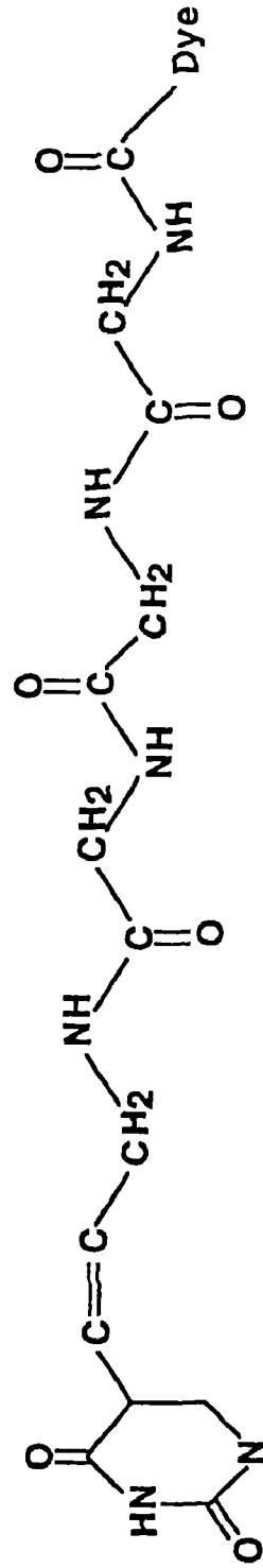
Tetraglycinyllinker
