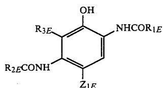
General Formula (E):
