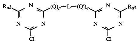
General Formula (HDB):
