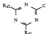
General Formula (HDA):
