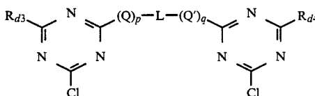
General Formula (HDB):
