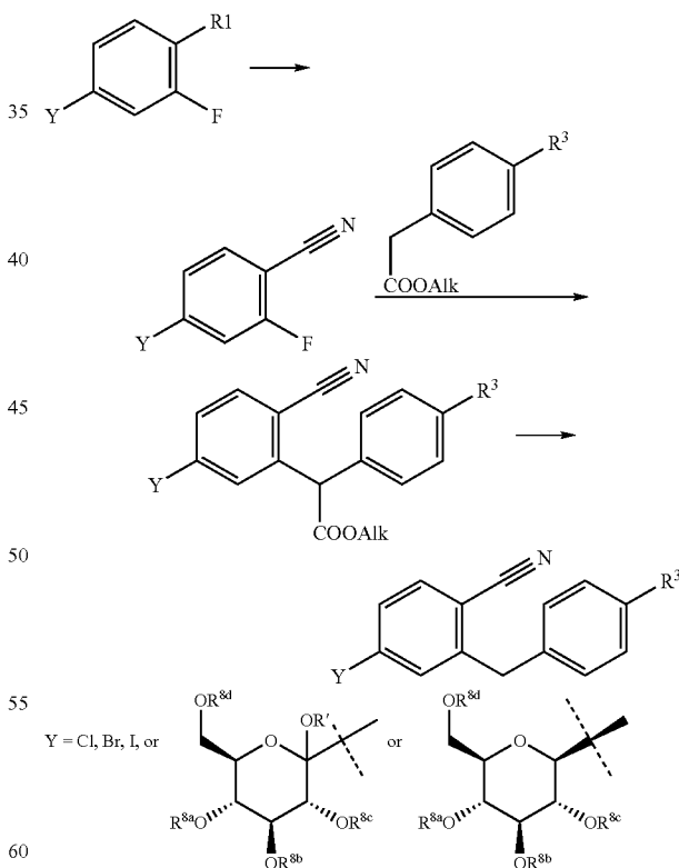
Scheme 8: Alternative Synthesis of Diarylmethane Unit
