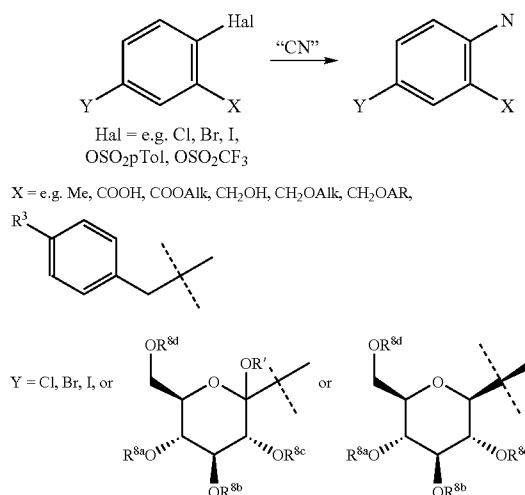
Scheme 5: Introduction of the Cyano Moiety
