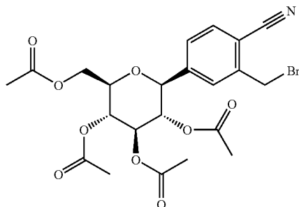
2-Bromomethyl-4-(2,3,4,6-tetra-O-acetyl-D-glucopyranos-1-yl)-benzonitrile
