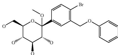
1-Bromo-4-(1-methoxy-D-glucopyranos-1-yl)-2-(phenoxymethyl)-benzene
