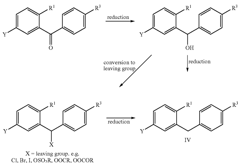
Scheme 3: Reduction of Diarylketones and Diarylmethanols to Diarylmethanes
