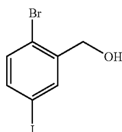
4-Bromo-3-hydroxymethyl-1-iodo-benzene
