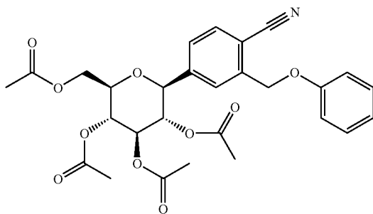
2-(Phenoxymethyl)-4-(2,3,4,6-tetra-O-acetyl-D-glucopyranos-1-yl)-benzonitrile
