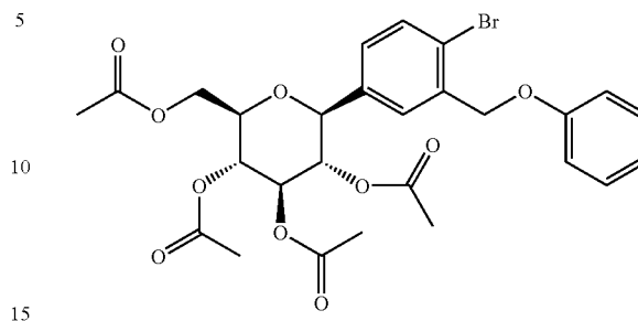
1-Bromo-4-(2,3,4,6-tetra-O-acetyl-D-glucopyranos-1-yl)-2-(phenoxymethyl)-benzene
