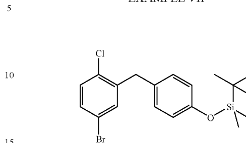
[4-(5-Bromo-2-chloro-benzyl)-phenoxy]-tert-butyl-dimethyl-silane
