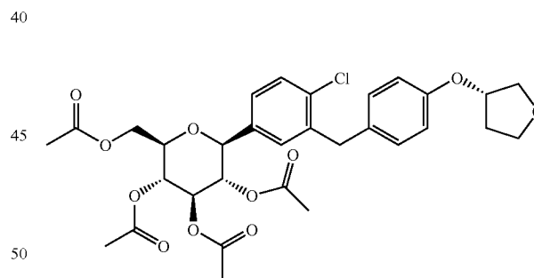
1-Chloro-2-[4-((S)-tetrahydrofuran-3-yloxy)-benzyl]-4-(2,3,4,6-tetra-O-acetyl-β-D-glucopyranos-1-yl)-benzene
