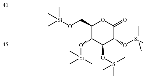
2,3,4,6-Tetrakis-O-(trimethylsilyl)-D-glucopyranone
