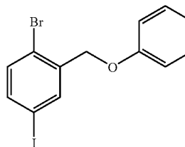
4-Bromo-1-iodo-3-phenoxy-methyl-benzene
