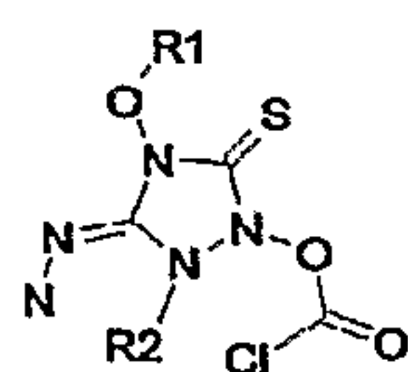
Library scaffold
