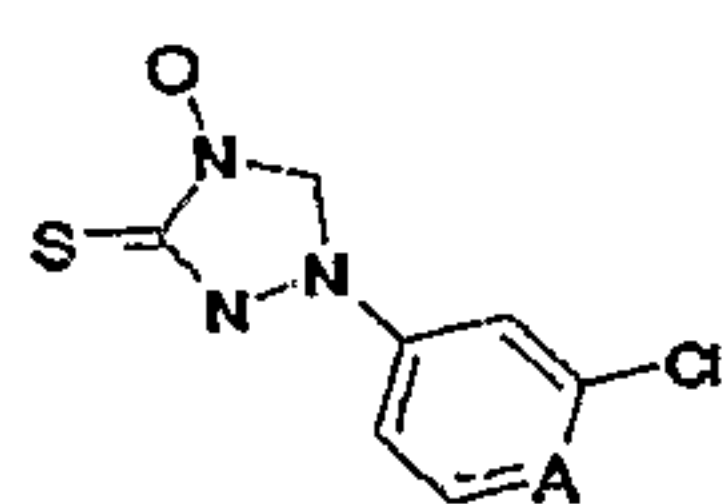
Query structure
