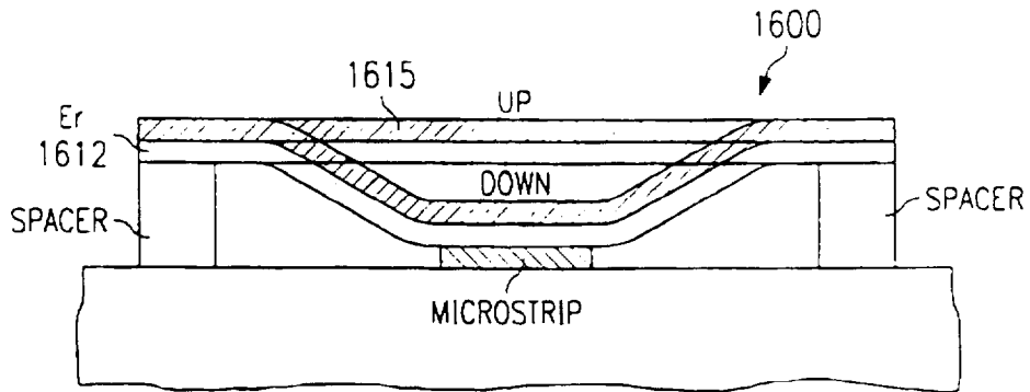
CAPACTIVE SWITCH METALLIZED DIELECTRIC MEMBRANE
