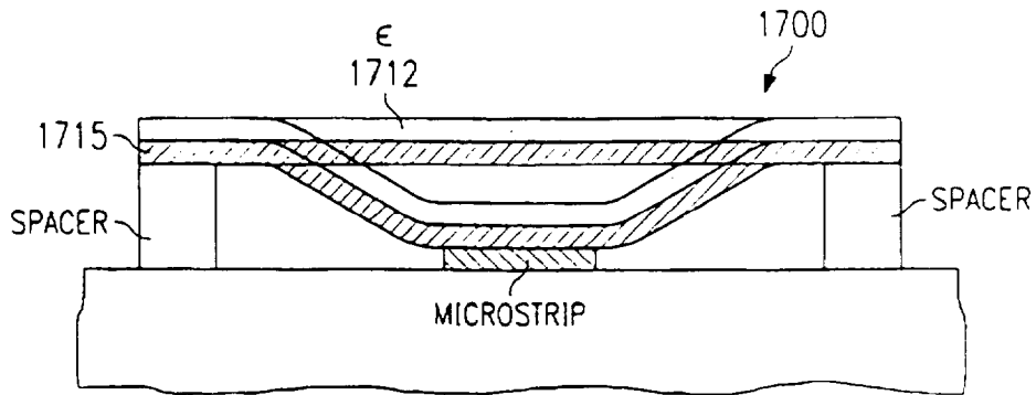
OHMIC SWITCH METALLIZED MEMBRANE
