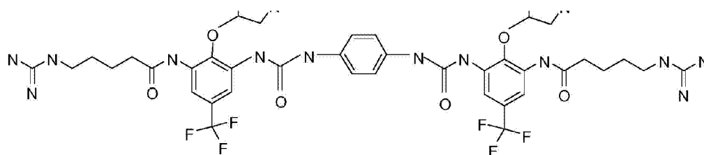
Compound Y,
