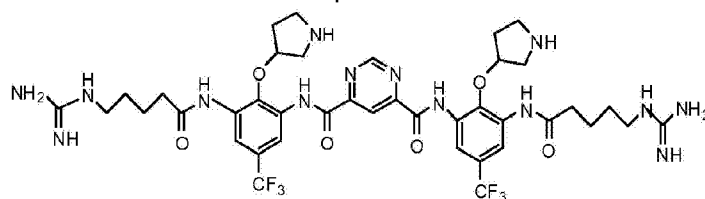
Compound X,
