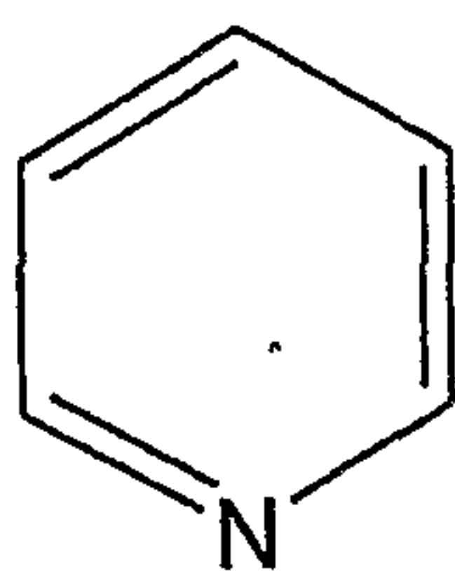
pyridine
