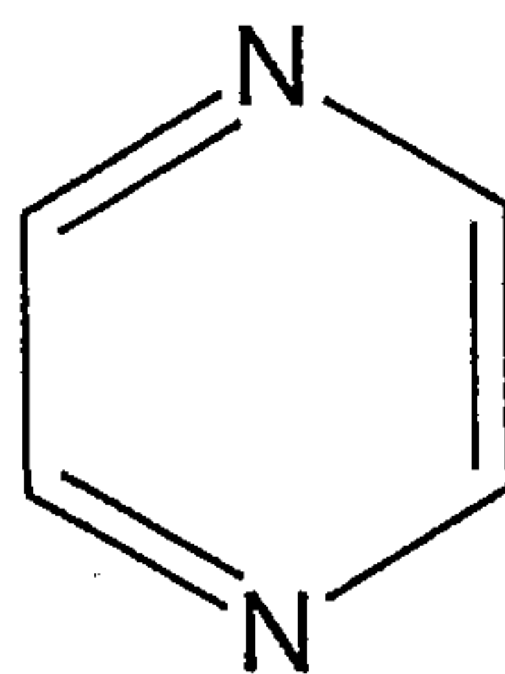
pyrazine
