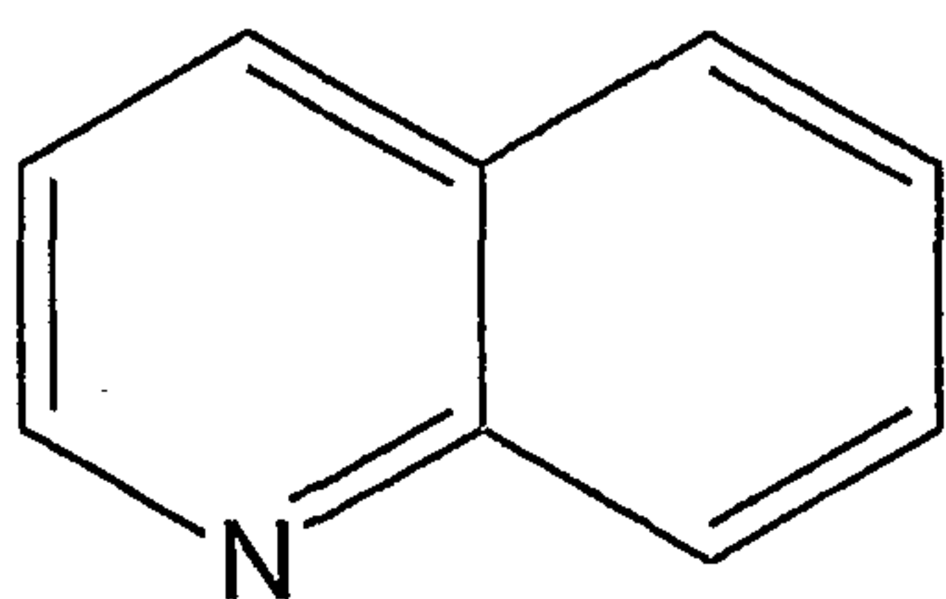
quinoline
