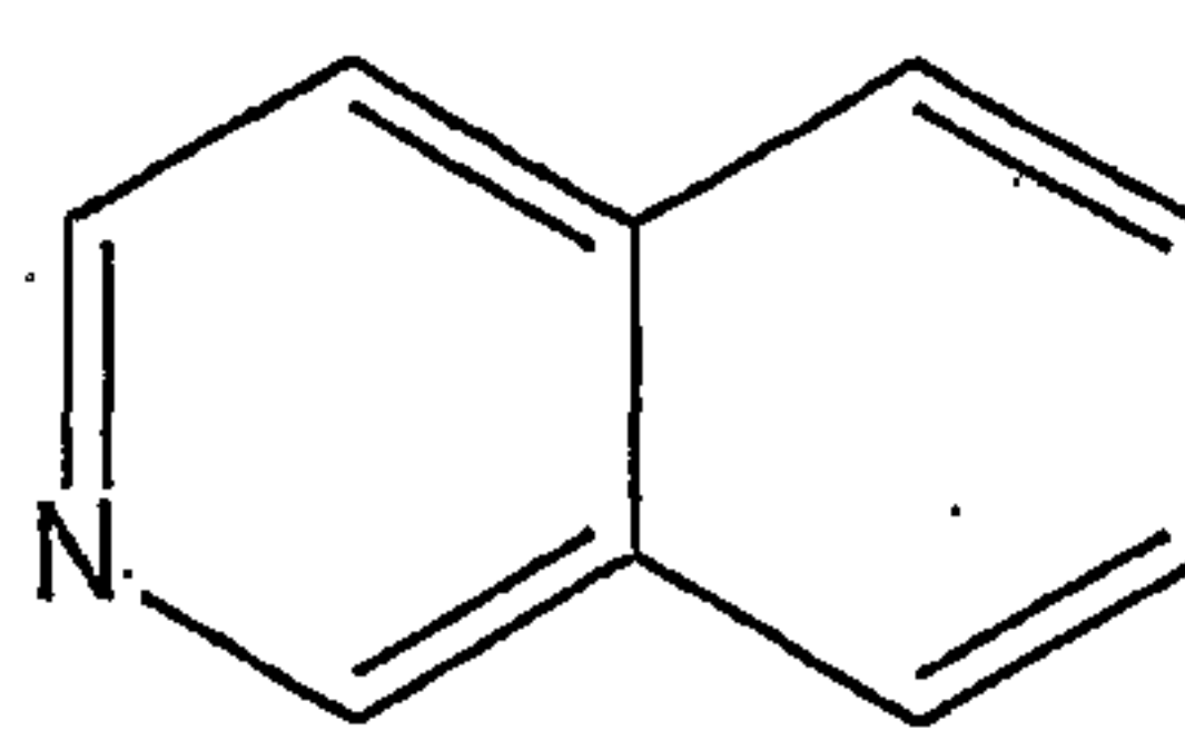
isoquinoline
