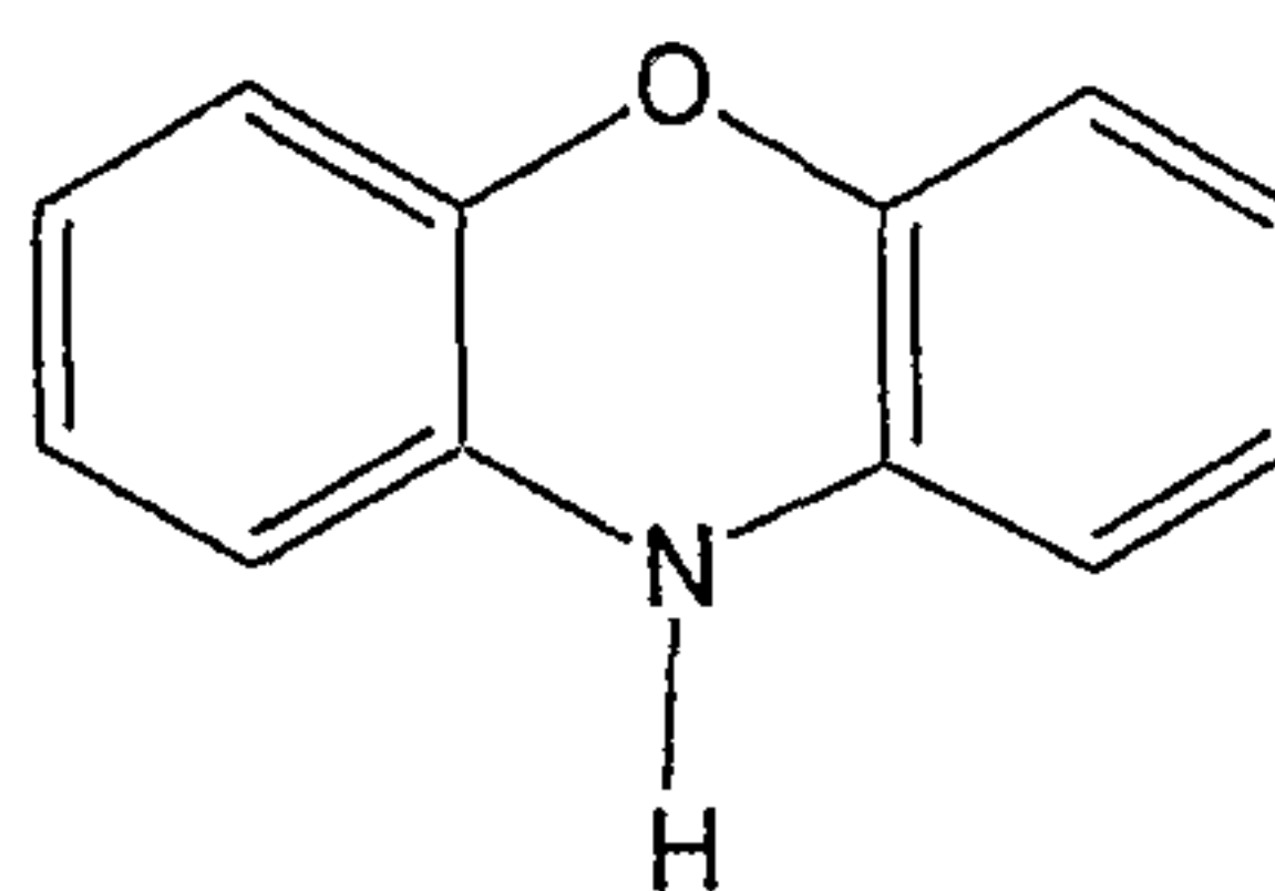
phenoxazine
