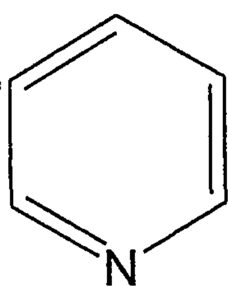
pyridine
