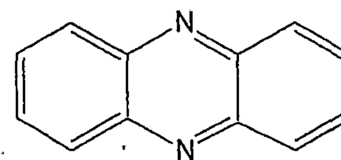
phenazine
