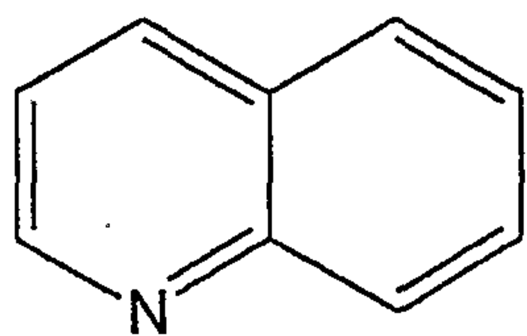
quinoline
