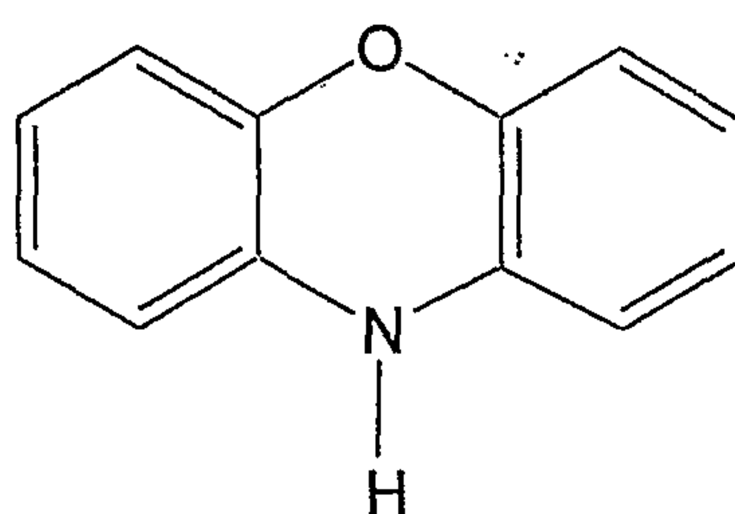
phenoxazine
