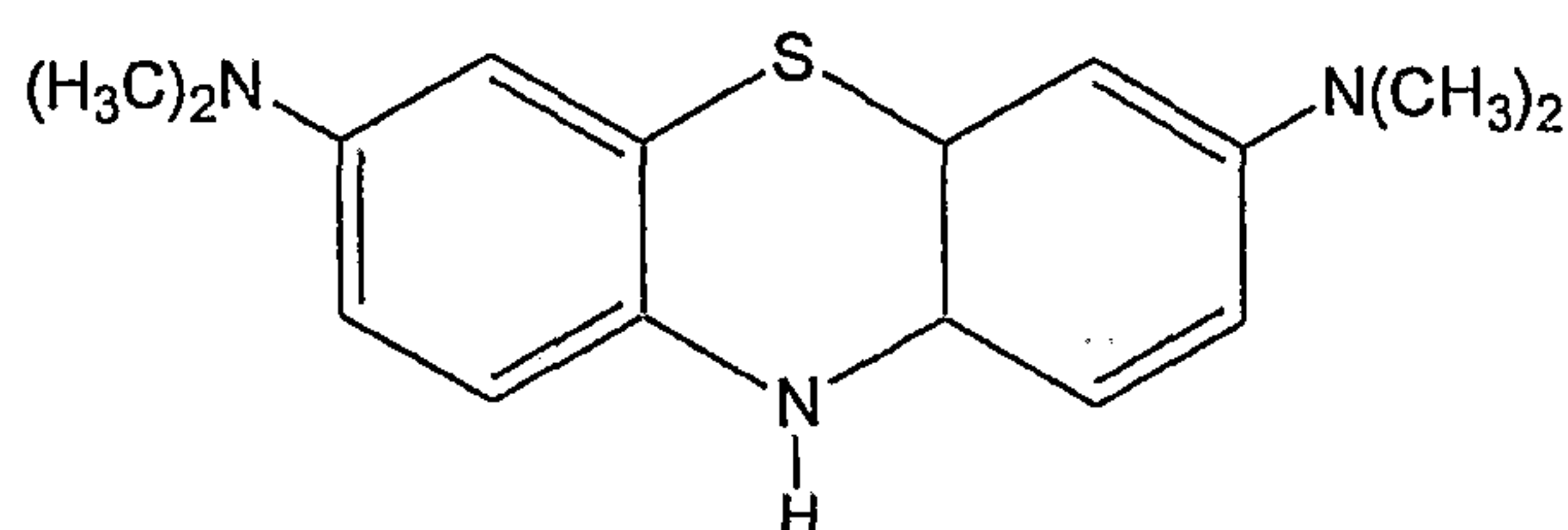
leucomethylene blue
