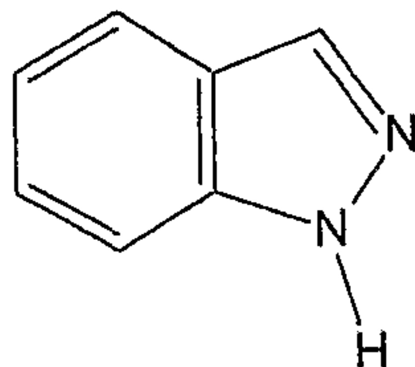
indazole
