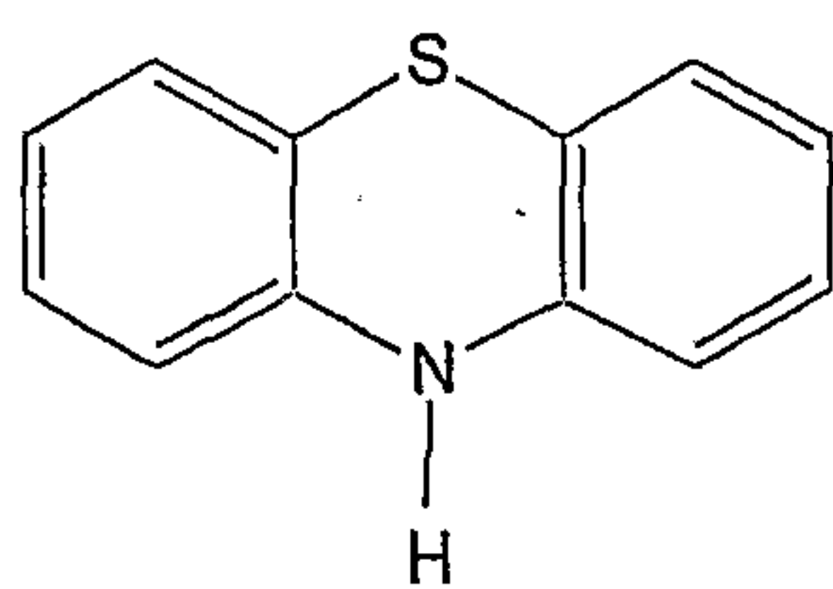
phenothiazine
