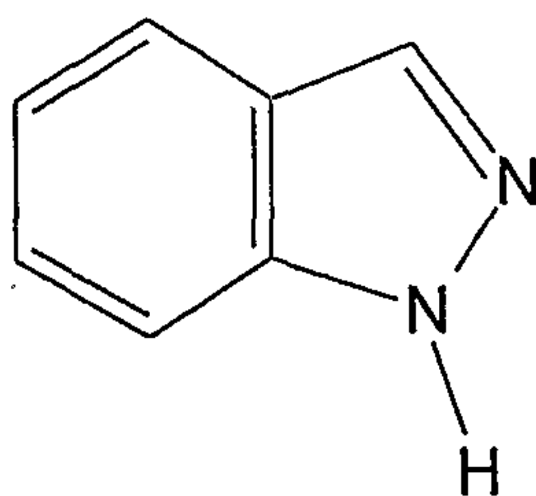
indazole
