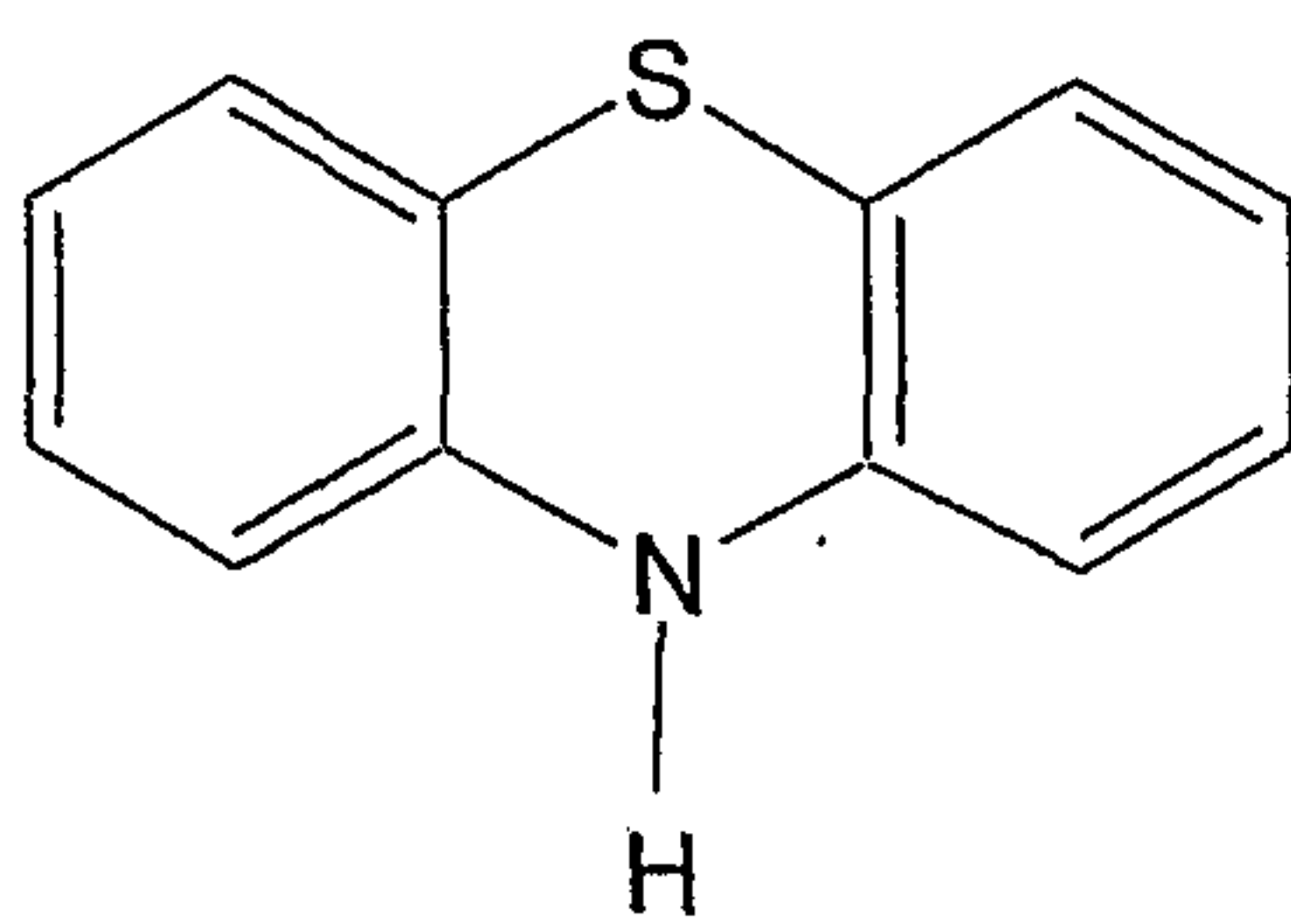
phenothiazine
