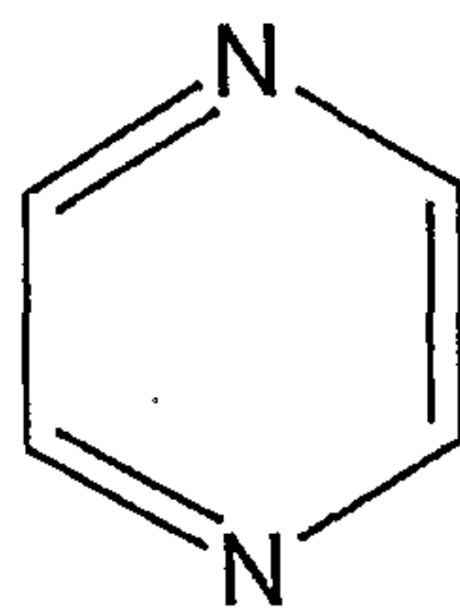
pyrazine
