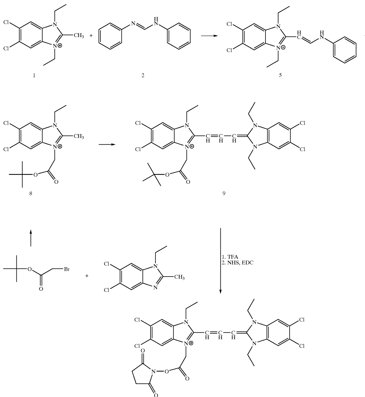
Scheme 2
