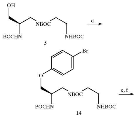
Scheme 2b: More Preferred Synthesis of Gd Complex 1
