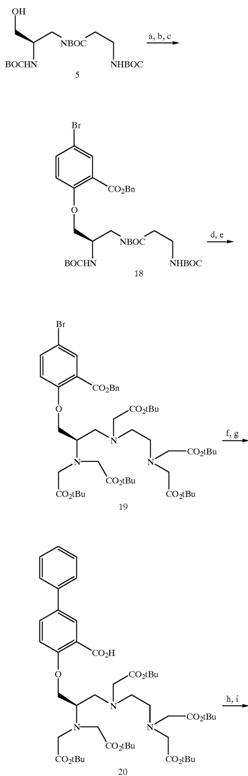
Scheme 3b: More Preferred Synthesis of Gd Complex 2
