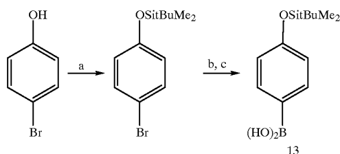
Scheme 2a: Synthesis of boronic acid 13
