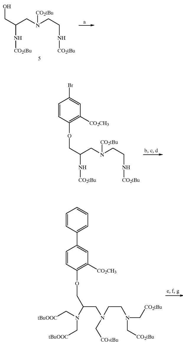
Scheme 3a: Synthesis of Gadolinium Complex 2
