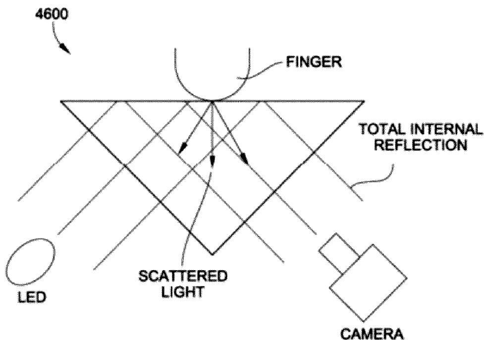
FIG. 46 PRIOR ART
