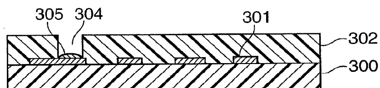
PRIOR ART FIG.4C
