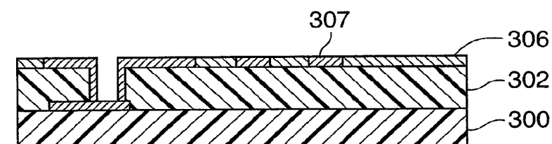
PRIOR ART FIG.4G
