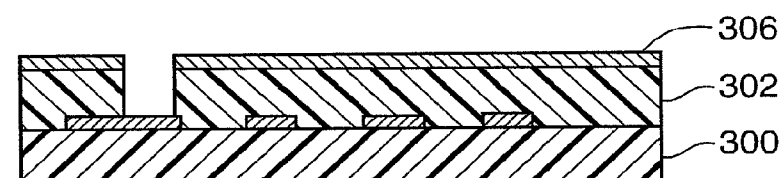
PRIOR ART FIG.4E
