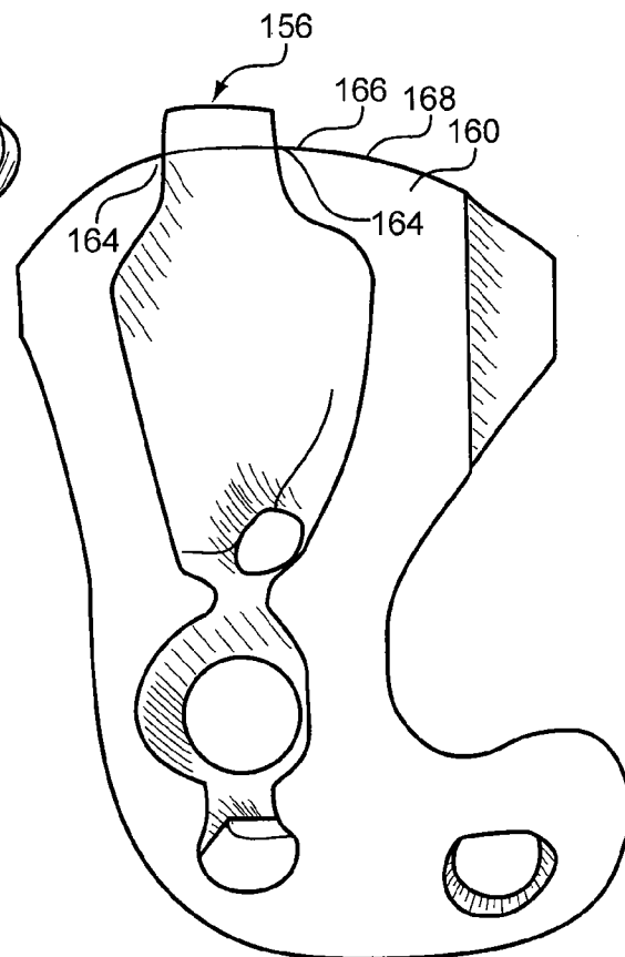
FIG. 27 PRIOR ART
