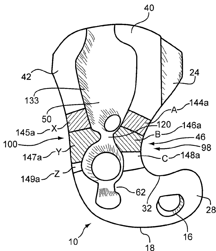
FIG. 16 PRIOR ART
