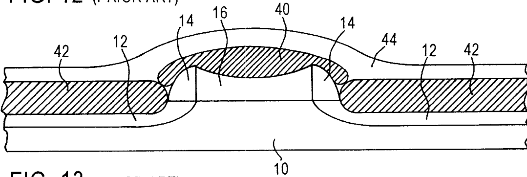
FIG. 13 (PRIOR ART)
