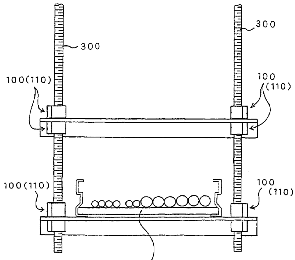
RECEIVING DEVICE FOR WIRING MATERIAL AND PIPING MATERIAL
